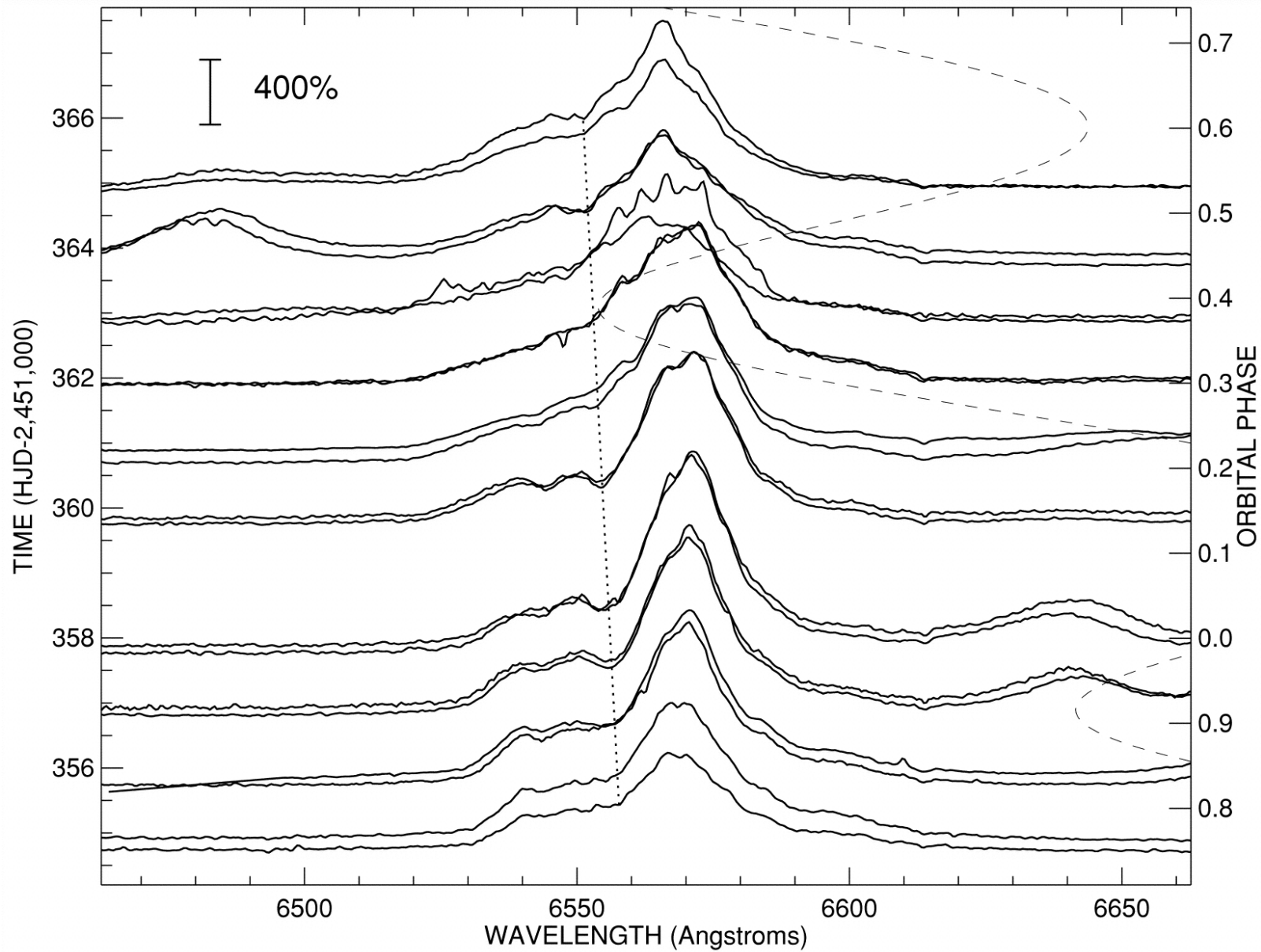
Fig. 6. from The Spectral Components of SS 433 Gies et al. 2002 ApJ 566 1069 doi:10.1086/338335 https://dx.doi.org/10.1086/338335
