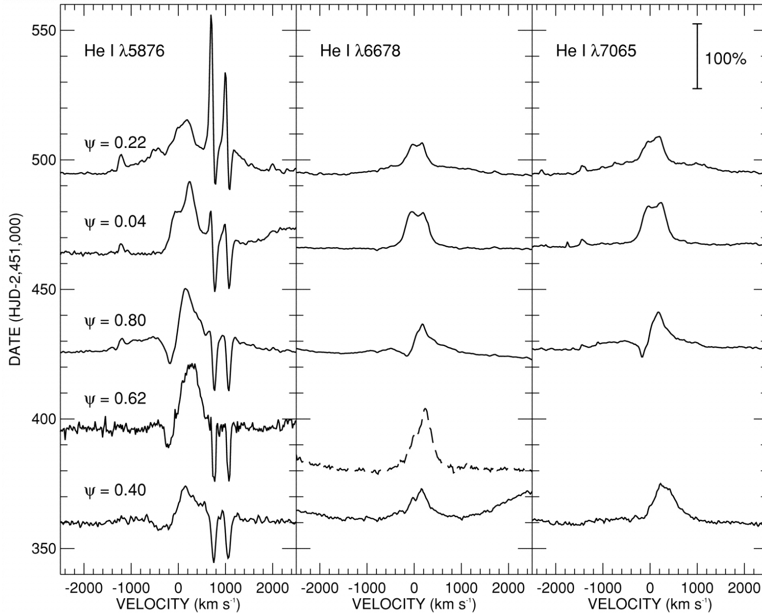
Fig. 5. from The Spectral Components of SS 433 Gies et al. 2002 ApJ 566 1069 doi:10.1086/338335 https://dx.doi.org/10.1086/338335
