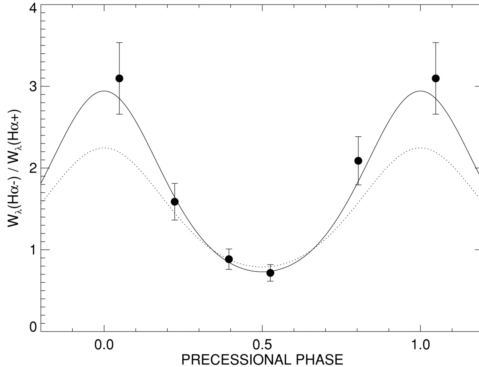
Fig. 3. from The Spectral Components of SS 433 Gies et al. 2002 ApJ 566 1069 doi:10.1086/338335 https://dx.doi.org/10.1086/338335
