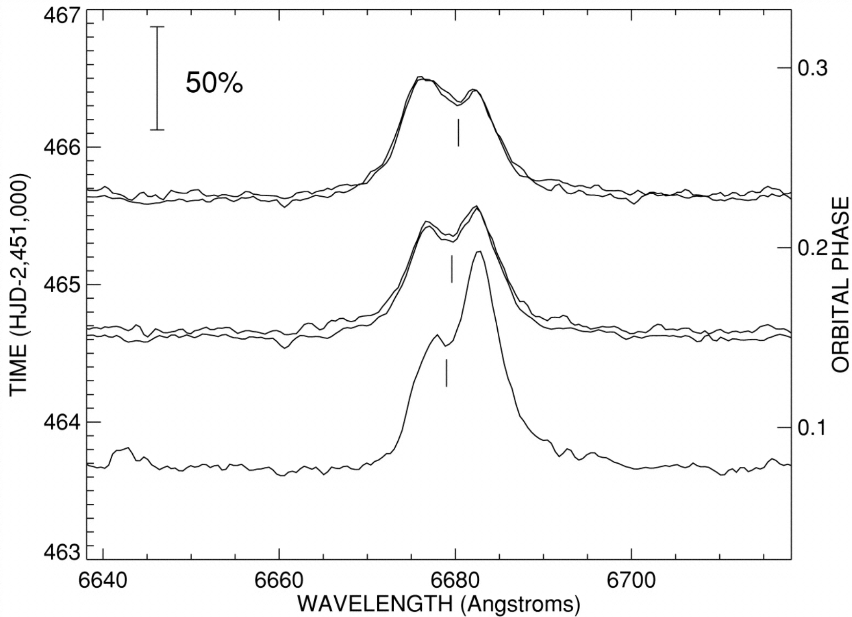
Fig. 13. from The Spectral Components of SS 433 Gies et al. 2002 ApJ 566 1069 doi:10.1086/338335 https://dx.doi.org/10.1086/338335
