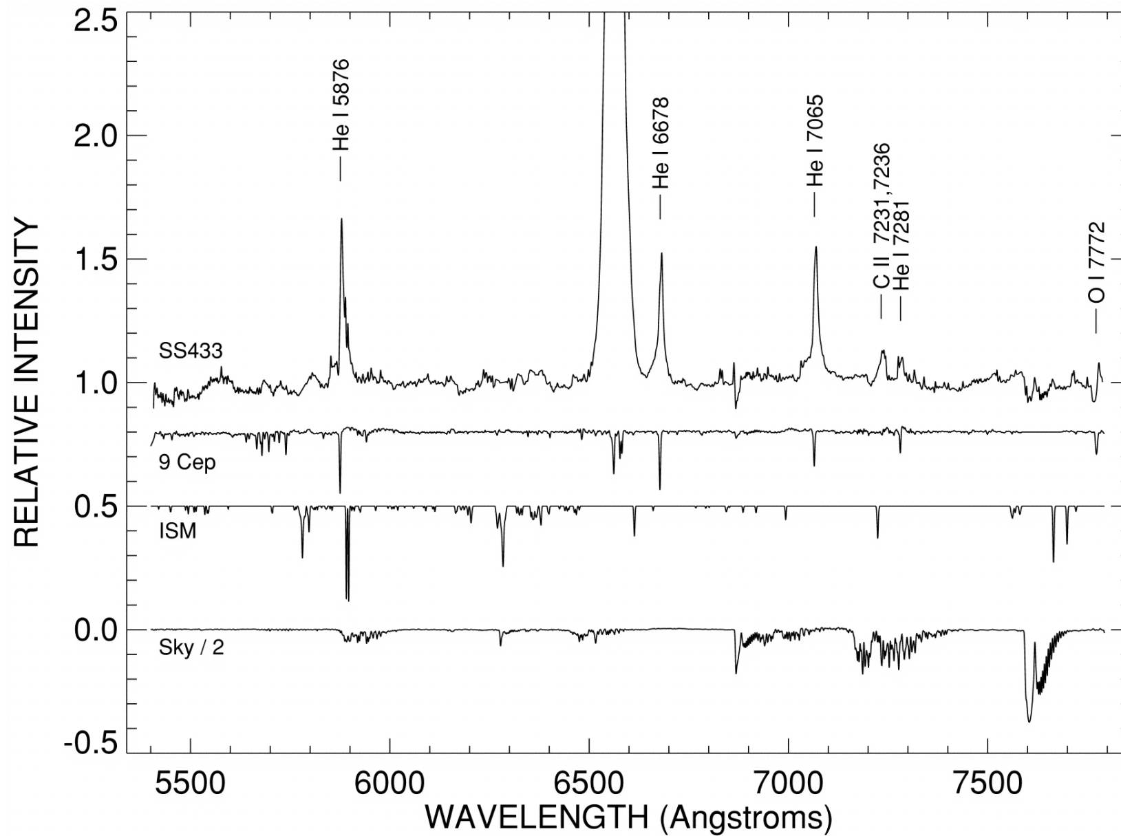
Fig. 10. from The Spectral Components of SS 433 Gies et al. 2002 ApJ 566 1069 doi:10.1086/338335 https://dx.doi.org/10.1086/338335
