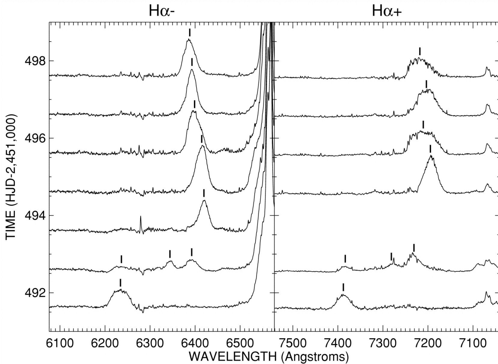
Fig. 1. from The Spectral Components of SS 433 Gies et al. 2002 ApJ 566 1069 doi:10.1086/338335 https://dx.doi.org/10.1086/338335
