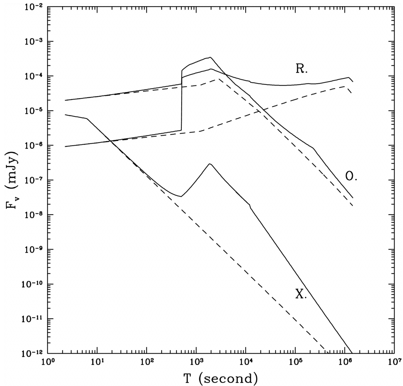
Fig. 5. from GammaRay Bursts with Continuous Energy Injection and Their Afterglow Signature Zhang & Mészáros 2002 ApJ 566 712 doi:10.1086/338247 https://dx.doi.org/10.1086/338247
