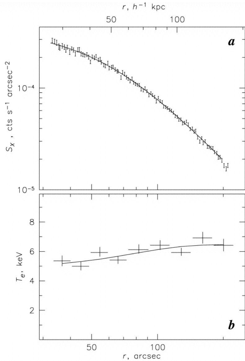
Fig. 3. from Nonhydrostatic Gas in the Core of the Relaxed Galaxy Cluster A1795 Markevitch, Vikhlinin, & Mazzotta 2001 ApJL 562 L153 doi:10.1086/337973 https://dx.doi.org/10.1086/337973 © 2001. The American Astronomical Society. All rights reserved. Printed in U.S.A.
