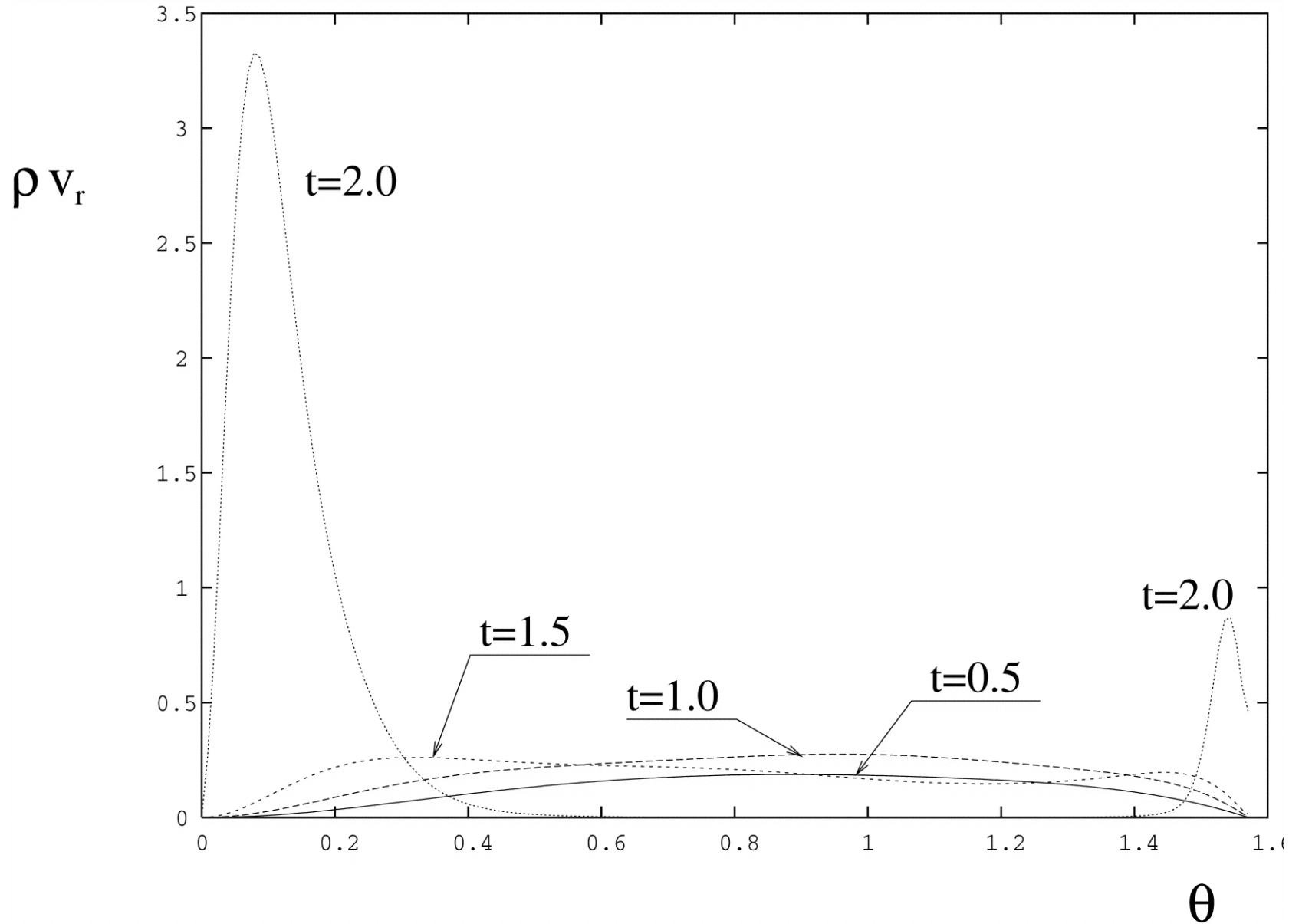
Fig. 2. from Magnetically Linked StarDisk Systems. II. Effects of Plasma Inertia and Reconnection in the Magnetosphere Uzdensky, Königl, & Litwin 2002 ApJ 565 1205 doi:10.1086/324724 https://dx.doi.org/10.1086/324724 © 2002. The American Astronomical Society. All rights reserved. Printed in U.S.A.
