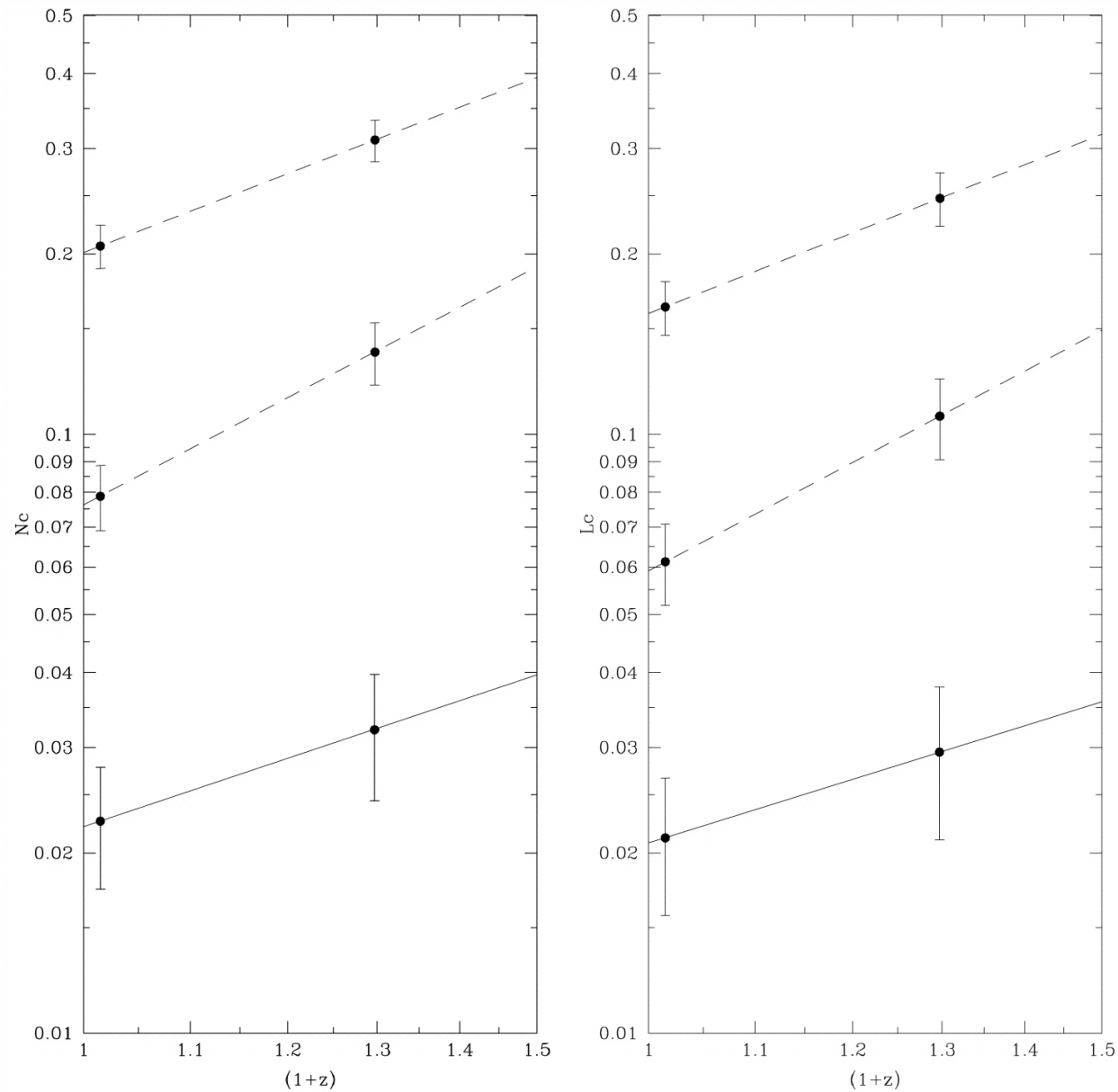
Fig. 8. from Dynamically Close Galaxy Pairs and Merger Rate Evolution in the CNOC2 Redshift Survey Patton et al. 2002 ApJ 565 208 doi:10.1086/324543 https://dx.doi.org/10.1086/324543 © 2002. The American Astronomical Society. All rights reserved. Printed in U.S.A.
