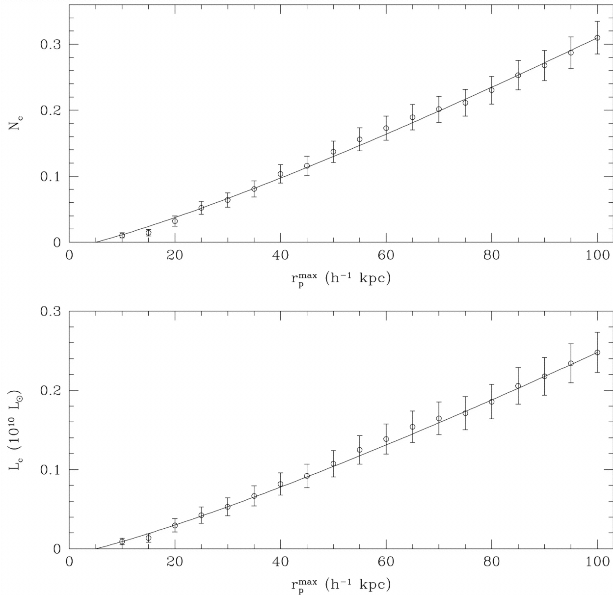
Fig. 6. from Dynamically Close Galaxy Pairs and Merger Rate Evolution in the CNOC2 Redshift Survey Patton et al. 2002 ApJ 565 208 doi:10.1086/324543 https://dx.doi.org/10.1086/324543 © 2002. The American Astronomical Society. All rights reserved. Printed in U.S.A.
