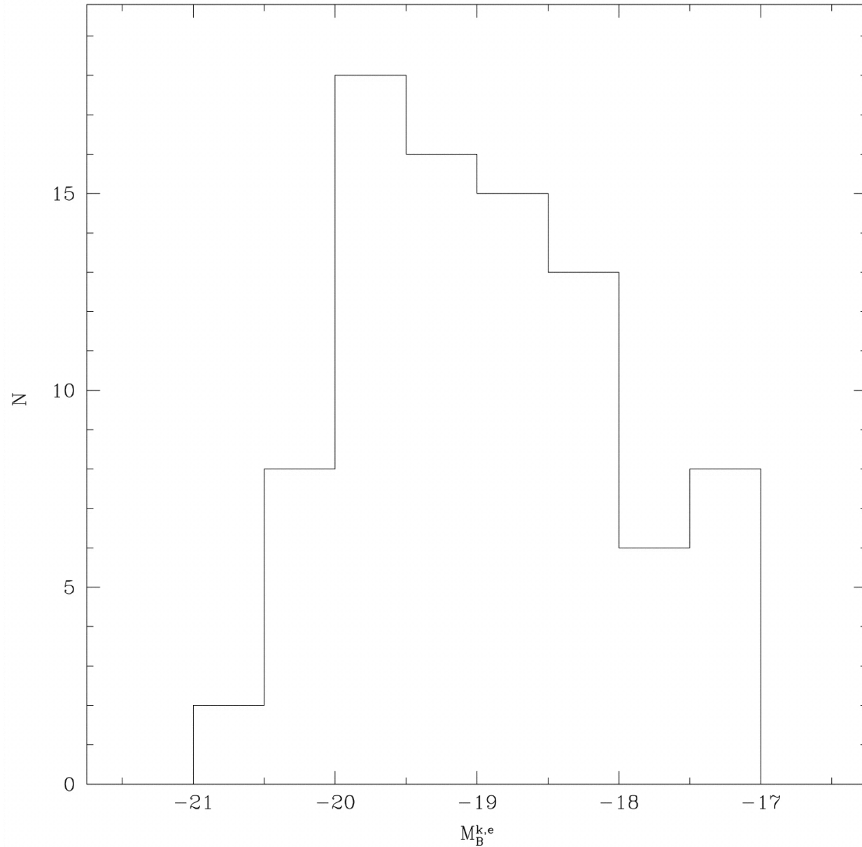
Fig. 4. from Dynamically Close Galaxy Pairs and Merger Rate Evolution in the CNOC2 Redshift Survey Patton et al. 2002 ApJ 565 208 doi:10.1086/324543 https://dx.doi.org/10.1086/324543 © 2002. The American Astronomical Society. All rights reserved. Printed in U.S.A.
