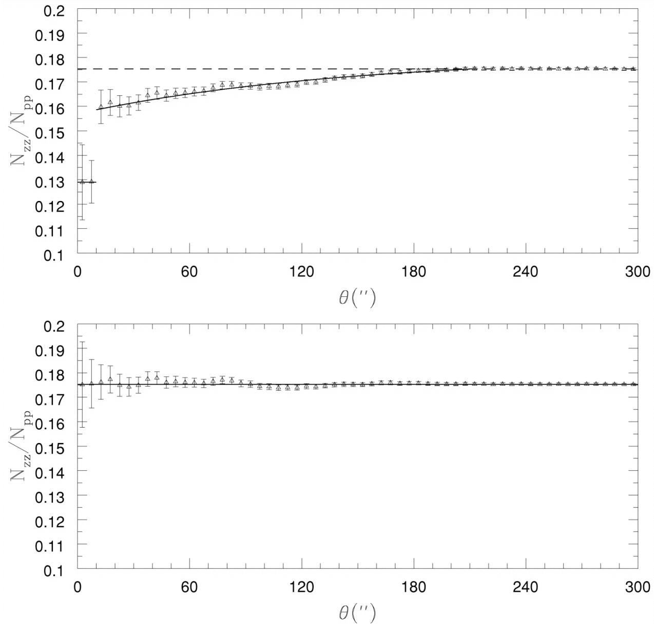
Fig. 3. from Dynamically Close Galaxy Pairs and Merger Rate Evolution in the CNOC2 Redshift Survey Patton et al. 2002 ApJ 565 208 doi:10.1086/324543 https://dx.doi.org/10.1086/324543
