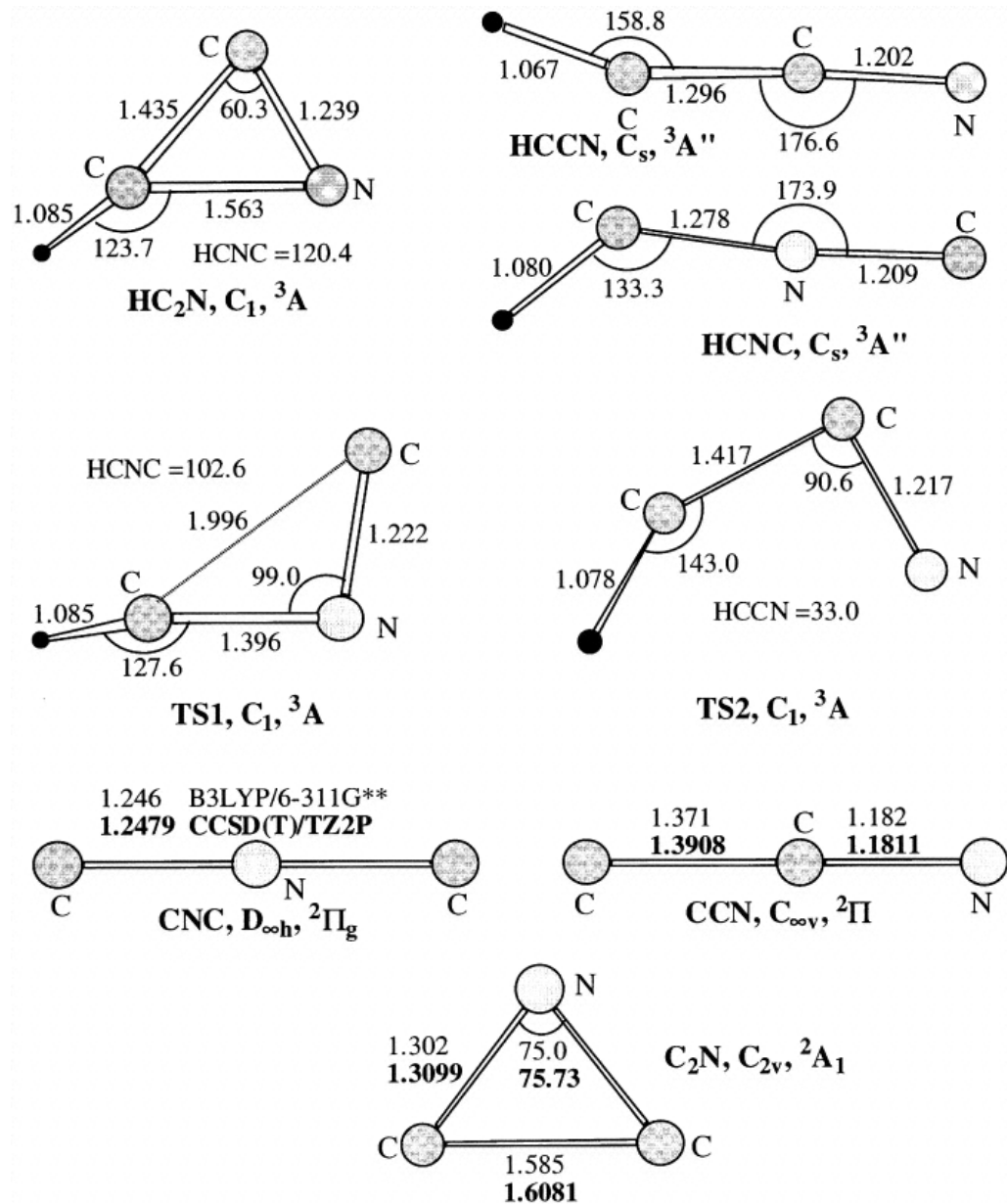
Fig. 2. from The Formation of Interstellar C 2 N Isomers in Circumstellar Envelopes of Carbon Stars: An Ab Initio Study Mebel & Kaiser 2002 ApJ 564 787 doi:10.1086/324334 https://dx.doi.org/10.1086/324334
