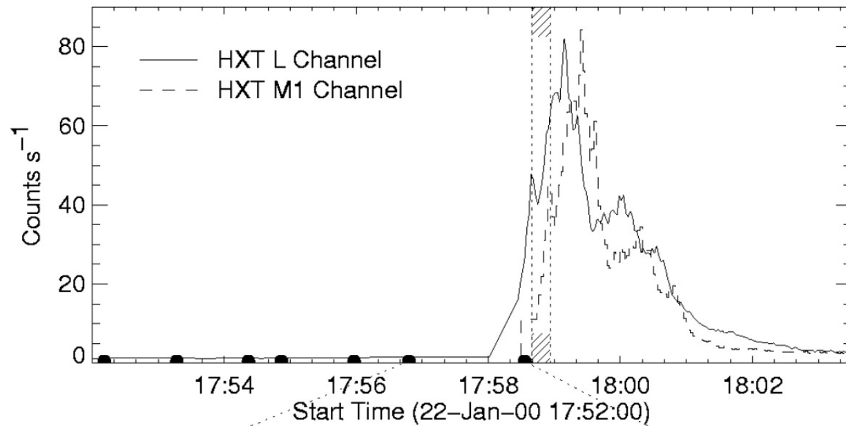
Fig. 4. from Ultraviolet Flare Ribbon Brightenings and the Onset of Hard XRay Emission Warren & Marshall 2001 ApJL 560 L87 doi:10.1086/324060 https://dx.doi.org/10.1086/324060 © 2001. The American Astronomical Society. All rights reserved. Printed in U.S.A.
