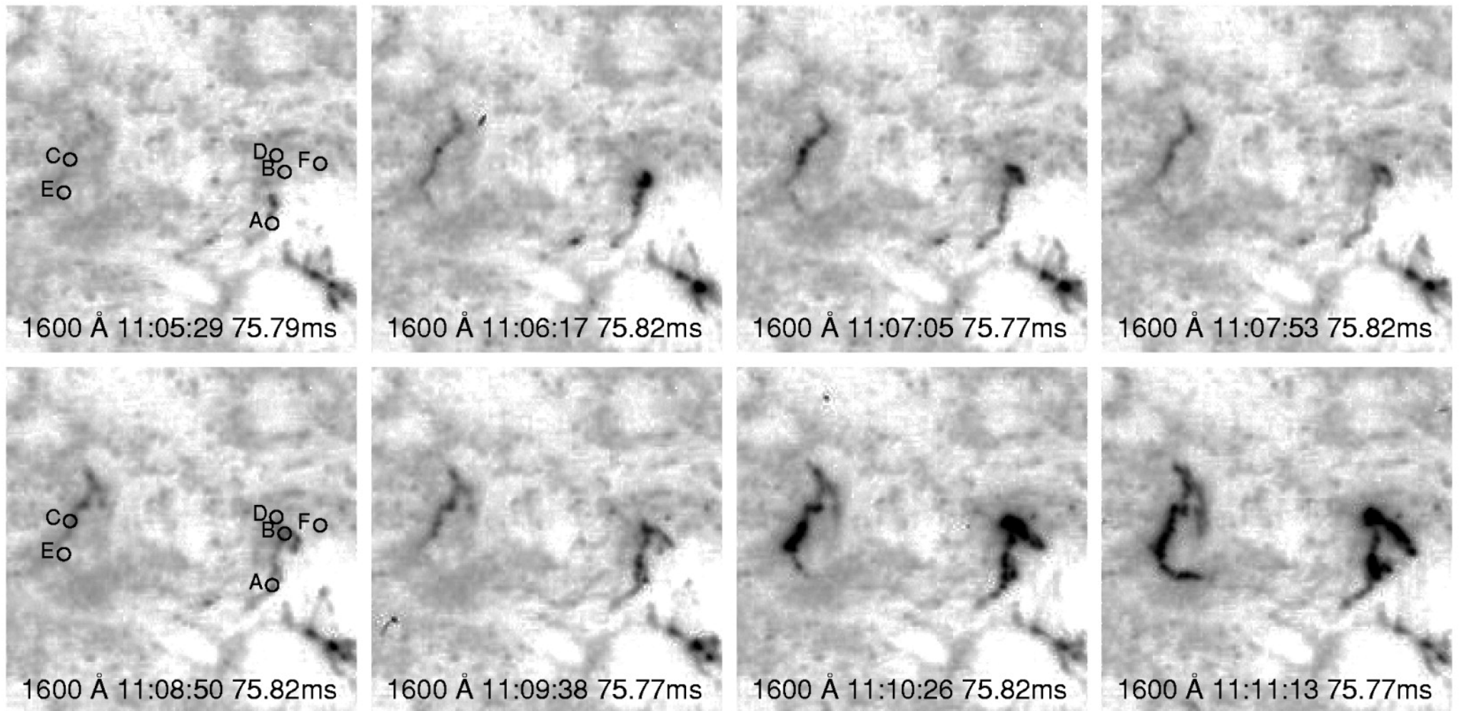
Fig. 1. from Ultraviolet Flare Ribbon Brightenings and the Onset of Hard XRay Emission Warren & Marshall 2001 ApJL 560 L87 doi:10.1086/324060 https://dx.doi.org/10.1086/324060 © 2001. The American Astronomical Society. All rights reserved. Printed in U.S.A.
