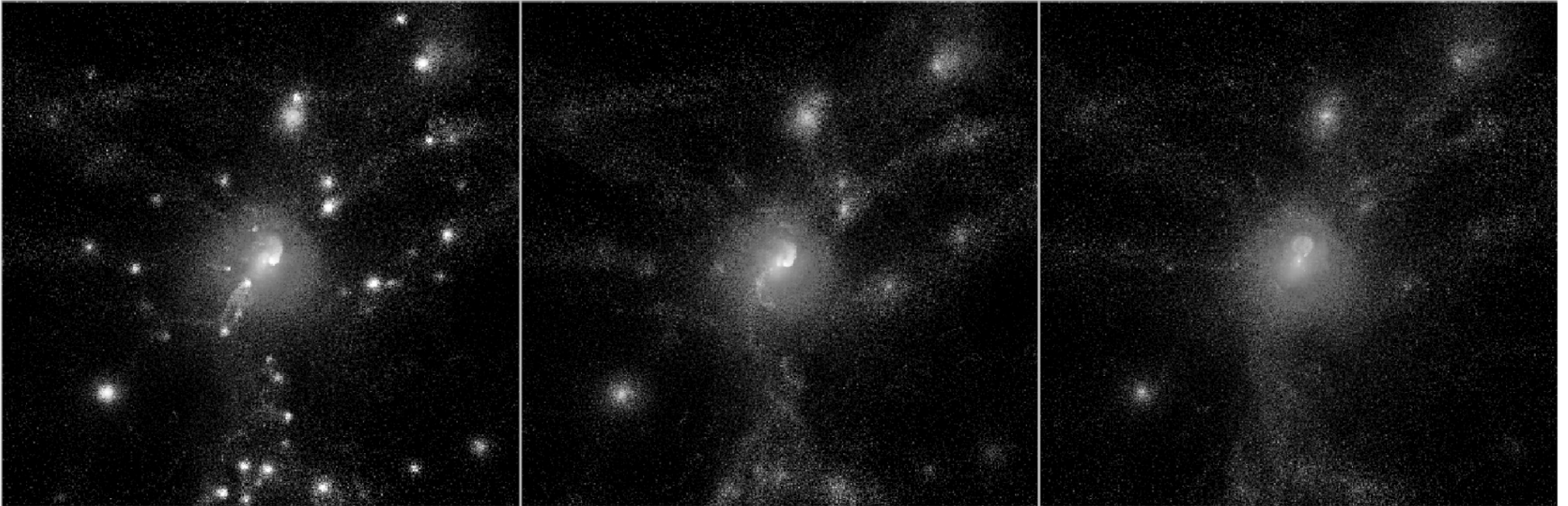
Fig. 1. from Preheating the Intracluster Medium in HighResolution Simulations: The Effect on the Gas Entropy Borgani et al. 2001 ApJL 559 L71 doi:10.1086/323905 https://dx.doi.org/10.1086/323905 © 2001. The American Astronomical Society. All rights reserved. Printed in U.S.A.
