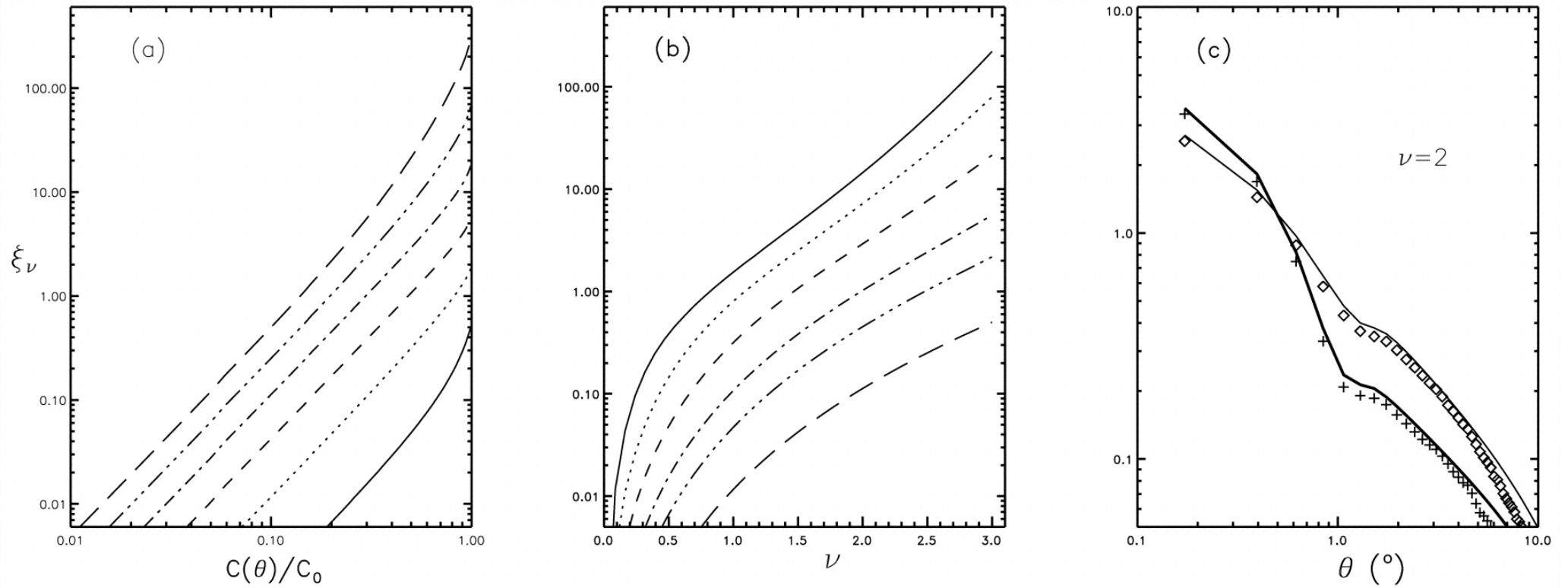
Fig. 1. from Determining Cosmic Microwave Background Structure from Its Peak Distribution Kashlinsky et al. 2001 ApJL 557 L1 doi:10.1086/323172 https://dx.doi.org/10.1086/323172 © 2001. The American Astronomical Society. All rights reserved. Printed in U.S.A.
