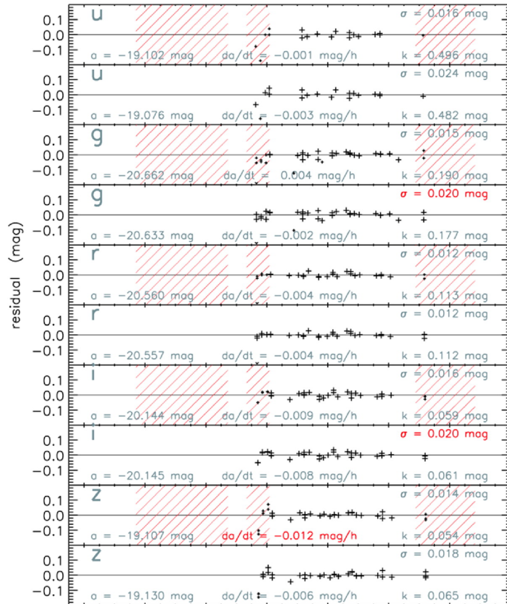
Fig. 5. from A Photometricity and Extinction Monitor at the Apache Point Observatory Hogg et al. 2001 AJ 122 2129 doi:10.1086/323103 https://dx.doi.org/10.1086/323103 © 2001. The American Astronomical Society. All rights reserved. Printed in U.S.A.
