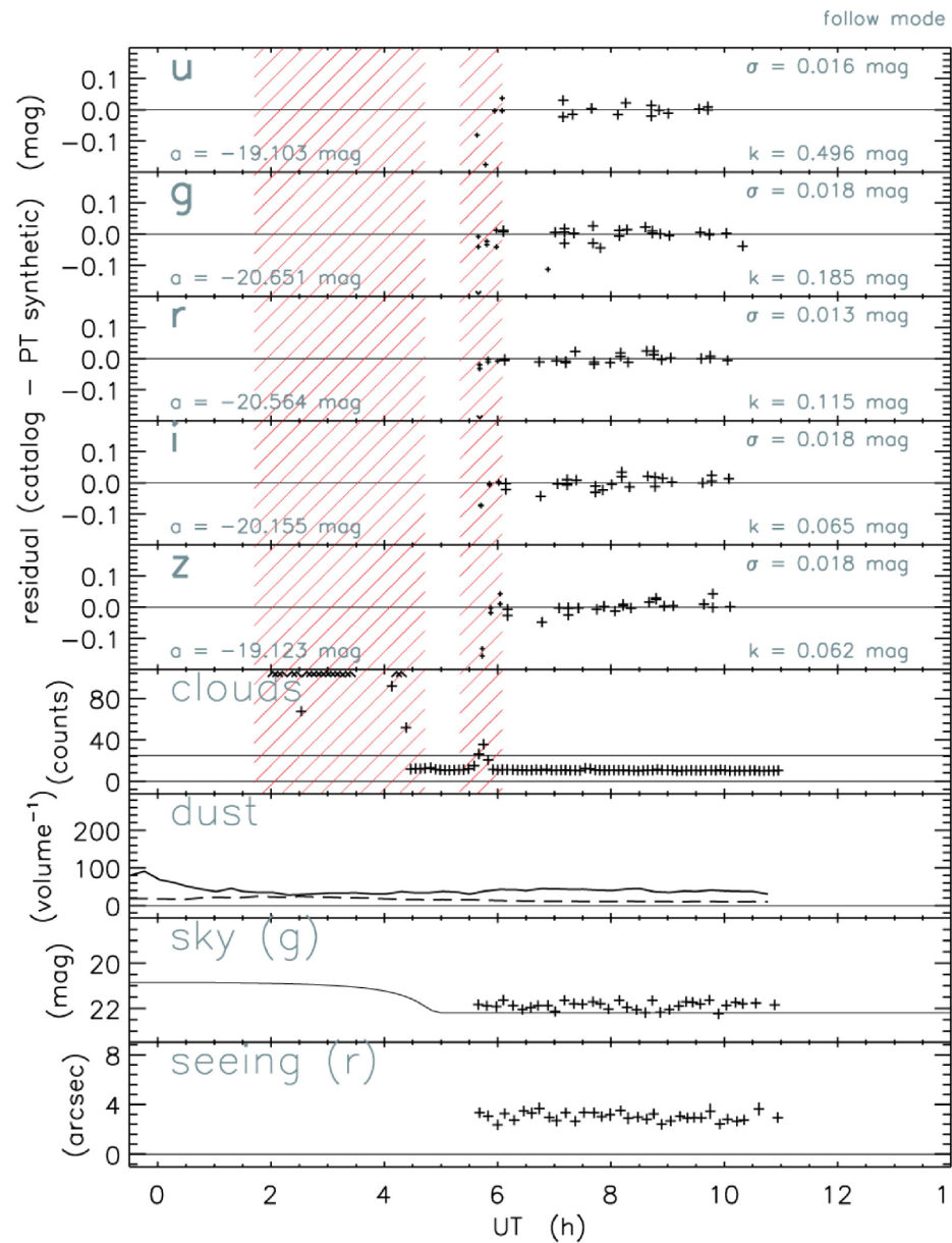
Fig. 4. from A Photometricity and Extinction Monitor at the Apache Point Observatory Hogg et al. 2001 AJ 122 2129 doi:10.1086/323103 https://dx.doi.org/10.1086/323103 © 2001. The American Astronomical Society. All rights reserved. Printed in U.S.A.
