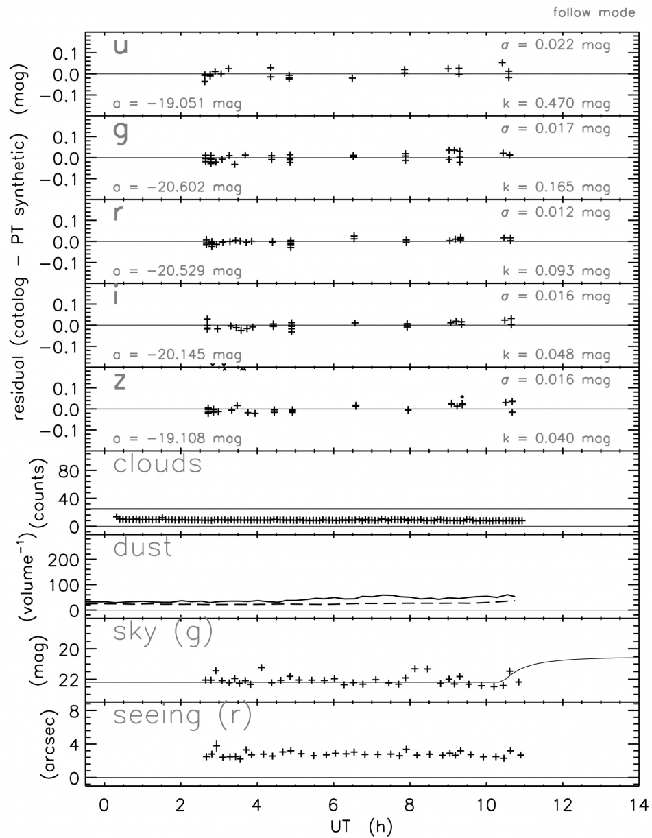
Fig. 3. from A Photometricity and Extinction Monitor at the Apache Point Observatory Hogg et al. 2001 AJ 122 2129 doi:10.1086/323103 https://dx.doi.org/10.1086/323103 © 2001. The American Astronomical Society. All rights reserved. Printed in U.S.A.
