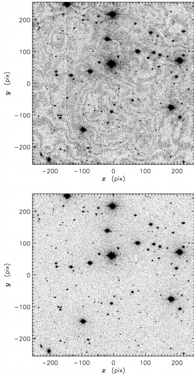
Fig. 1. from A Photometricity and Extinction Monitor at the Apache Point Observatory Hogg et al. 2001 AJ 122 2129 doi:10.1086/323103 https://dx.doi.org/10.1086/323103 © 2001. The American Astronomical Society. All rights reserved. Printed in U.S.A.
