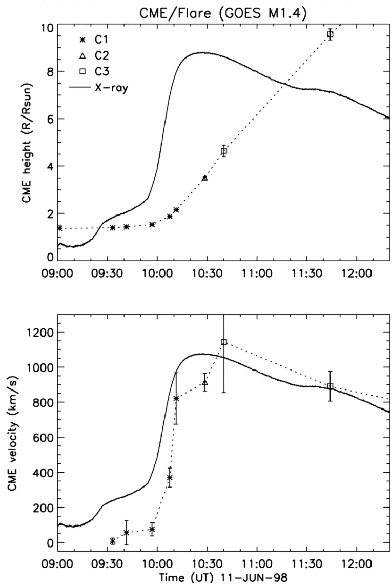
Fig. 2. from On the Temporal Relationship between Coronal Mass Ejections and Flares Zhang et al. 2001 ApJ 559 452 doi:10.1086/322405 https://dx.doi.org/10.1086/322405 © 2001. The American Astronomical Society. All rights reserved. Printed in U.S.A.
