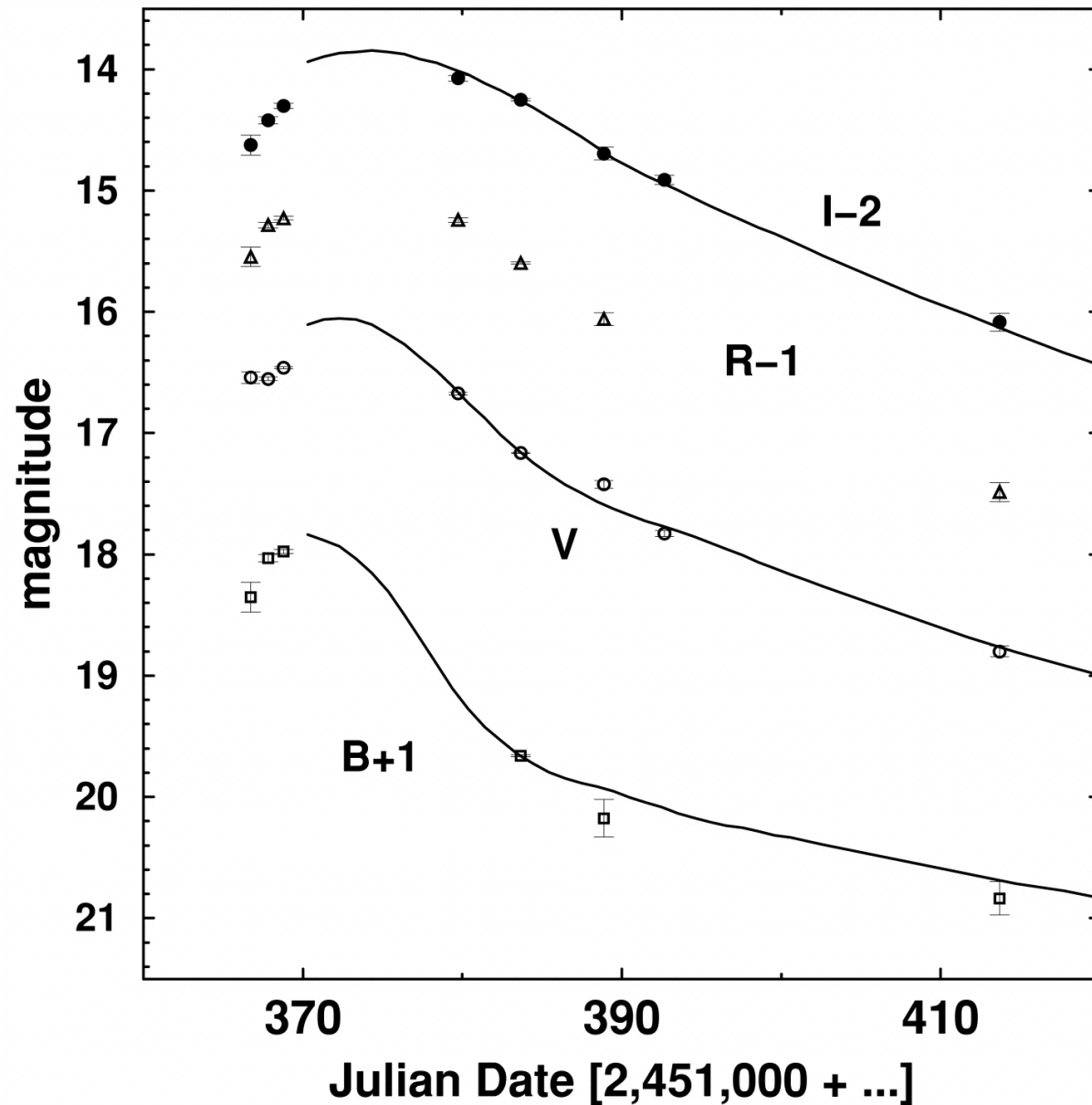
Fig. 6. from Optical and Infrared Photometry of the Type Ia Supernovae 1999da, 1999dk, 1999gp, 2000bk, and 2000ce Krisciunas et al. 2001 AJ 122 1616 doi:10.1086/322120 https://dx.doi.org/10.1086/322120 © 2001. The American Astronomical Society. All rights reserved. Printed in U.S.A.
