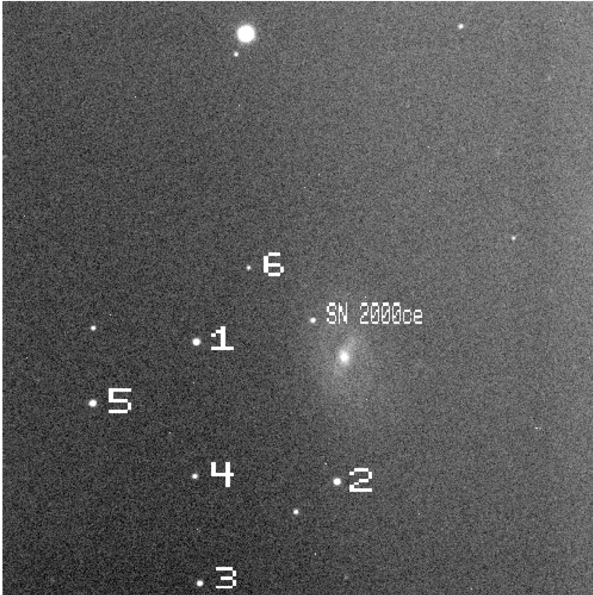
Fig. 5. from Optical and Infrared Photometry of the Type Ia Supernovae 1999da, 1999dk, 1999gp, 2000bk, and 2000ce Krisciunas et al. 2001 AJ 122 1616 doi:10.1086/322120 https://dx.doi.org/10.1086/322120 © 2001. The American Astronomical Society. All rights reserved. Printed in U.S.A.
