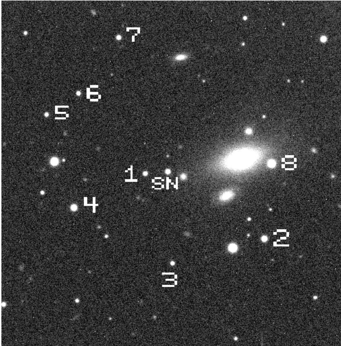
Fig. 4. from Optical and Infrared Photometry of the Type Ia Supernovae 1999da, 1999dk, 1999gp, 2000bk, and 2000ce Krisciunas et al. 2001 AJ 122 1616 doi:10.1086/322120 https://dx.doi.org/10.1086/322120
