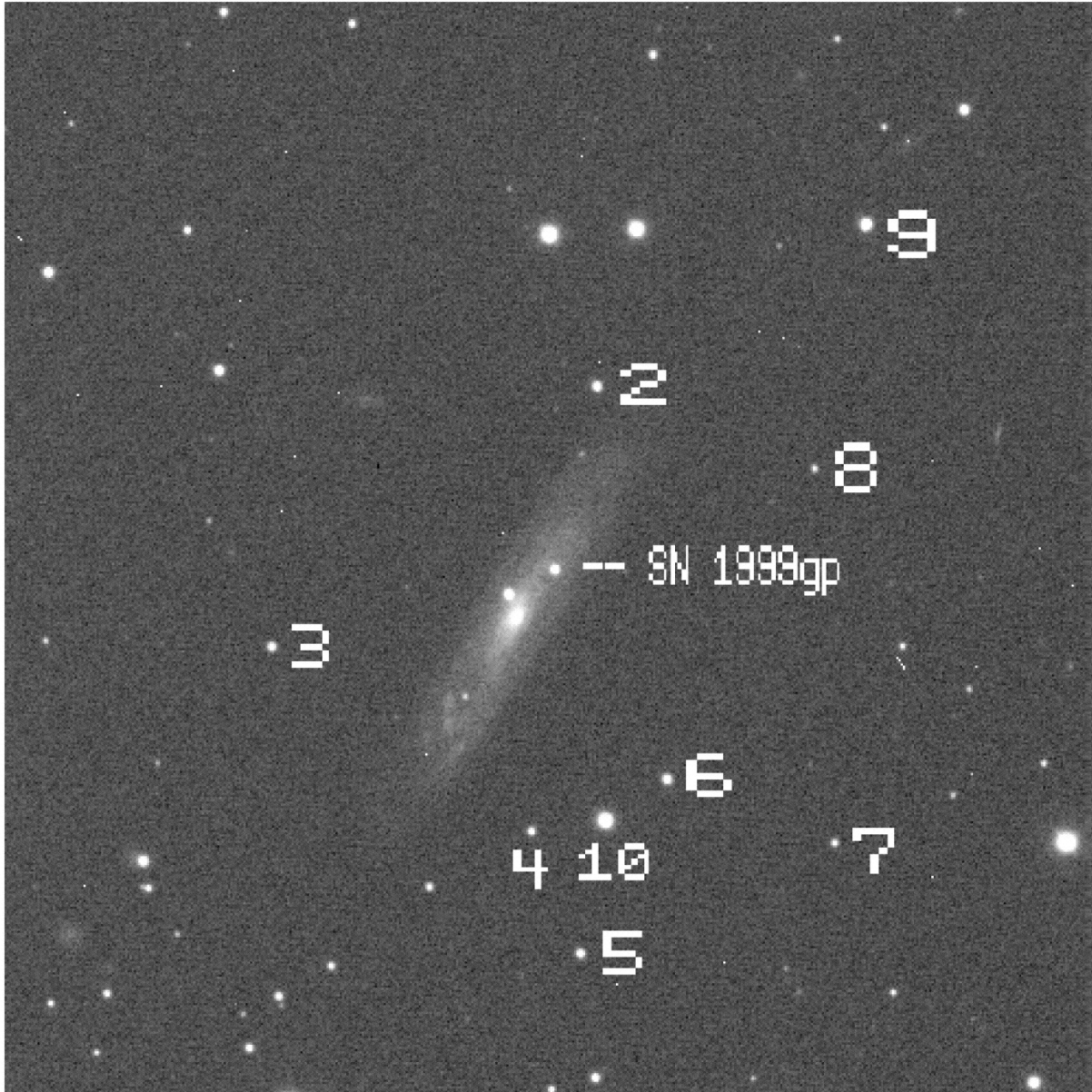
Fig. 3. from Optical and Infrared Photometry of the Type Ia Supernovae 1999da, 1999dk, 1999gp, 2000bk, and 2000ce Krisciunas et al. 2001 AJ 122 1616 doi:10.1086/322120 https://dx.doi.org/10.1086/322120
