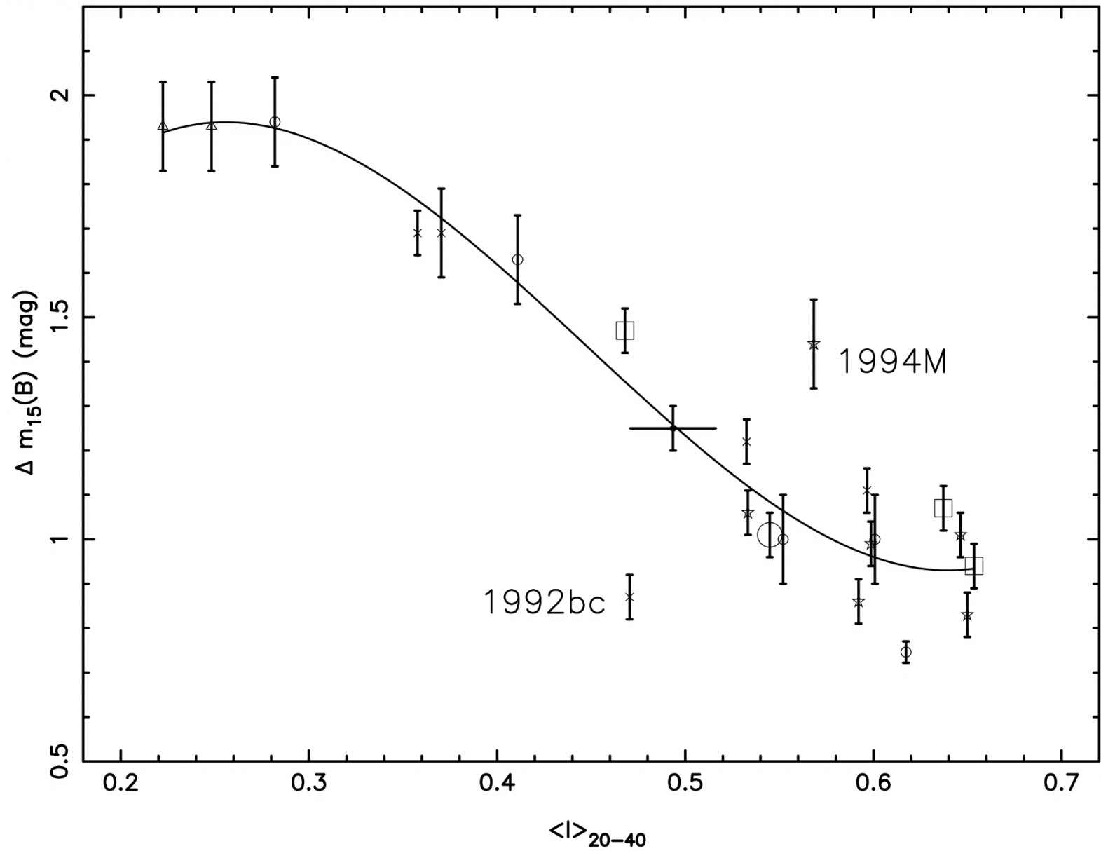
Fig. 17. from Optical and Infrared Photometry of the Type Ia Supernovae 1999da, 1999dk, 1999gp, 2000bk, and 2000ce Krisciunas et al. 2001 AJ 122 1616 doi:10.1086/322120 https://dx.doi.org/10.1086/322120 © 2001. The American Astronomical Society. All rights reserved. Printed in U.S.A.
