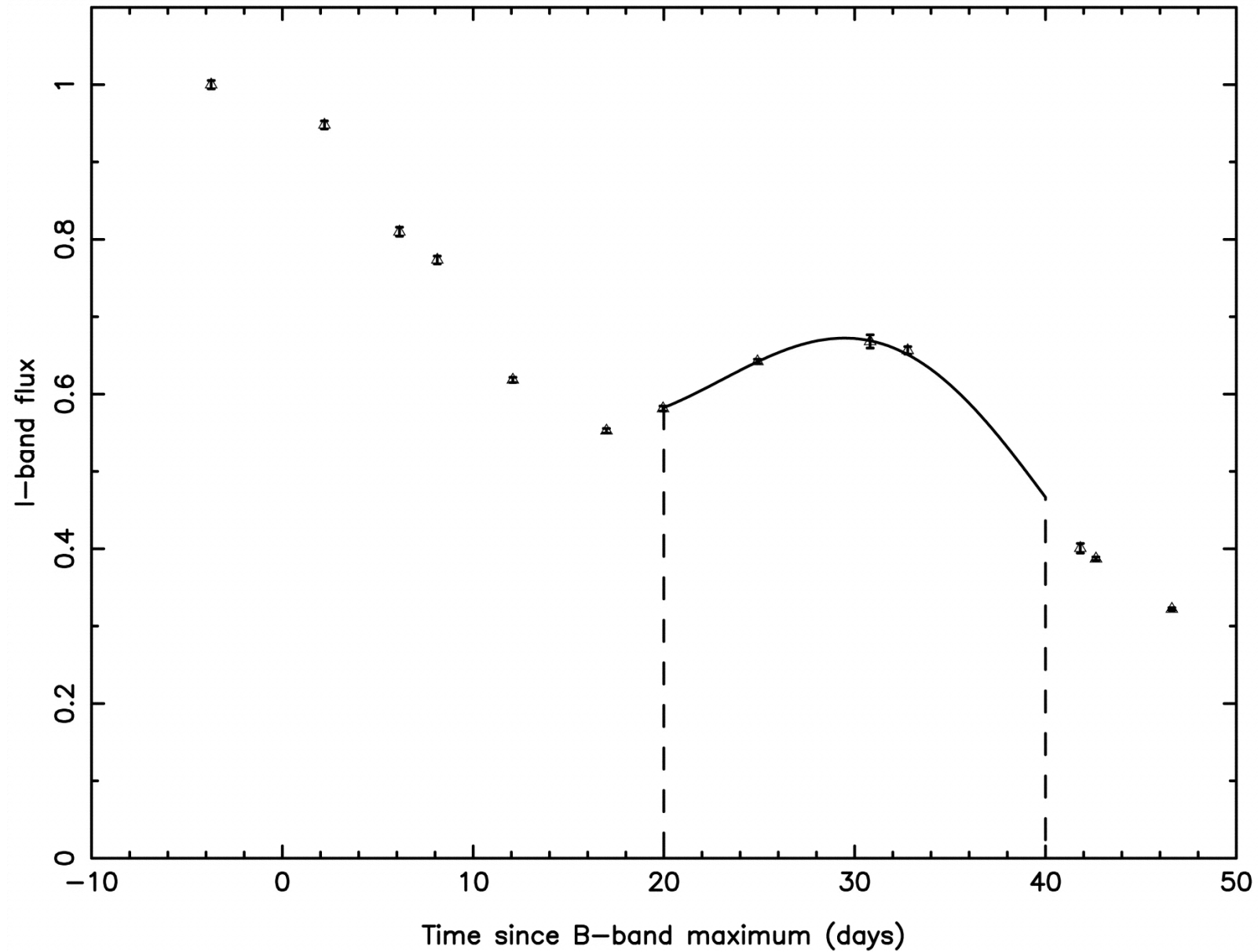
Fig. 16. from Optical and Infrared Photometry of the Type Ia Supernovae 1999da, 1999dk, 1999gp, 2000bk, and 2000ce Krisciunas et al. 2001 AJ 122 1616 doi:10.1086/322120 https://dx.doi.org/10.1086/322120 © 2001. The American Astronomical Society. All rights reserved. Printed in U.S.A.
