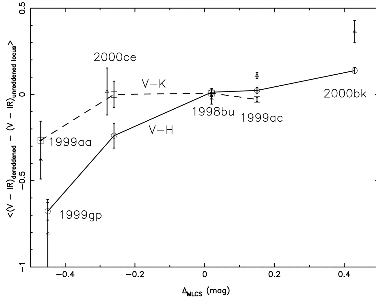
Fig. 15. from Optical and Infrared Photometry of the Type Ia Supernovae 1999da, 1999dk, 1999gp, 2000bk, and 2000ce Krisciunas et al. 2001 AJ 122 1616 doi:10.1086/322120 https://dx.doi.org/10.1086/322120 © 2001. The American Astronomical Society. All rights reserved. Printed in U.S.A.
