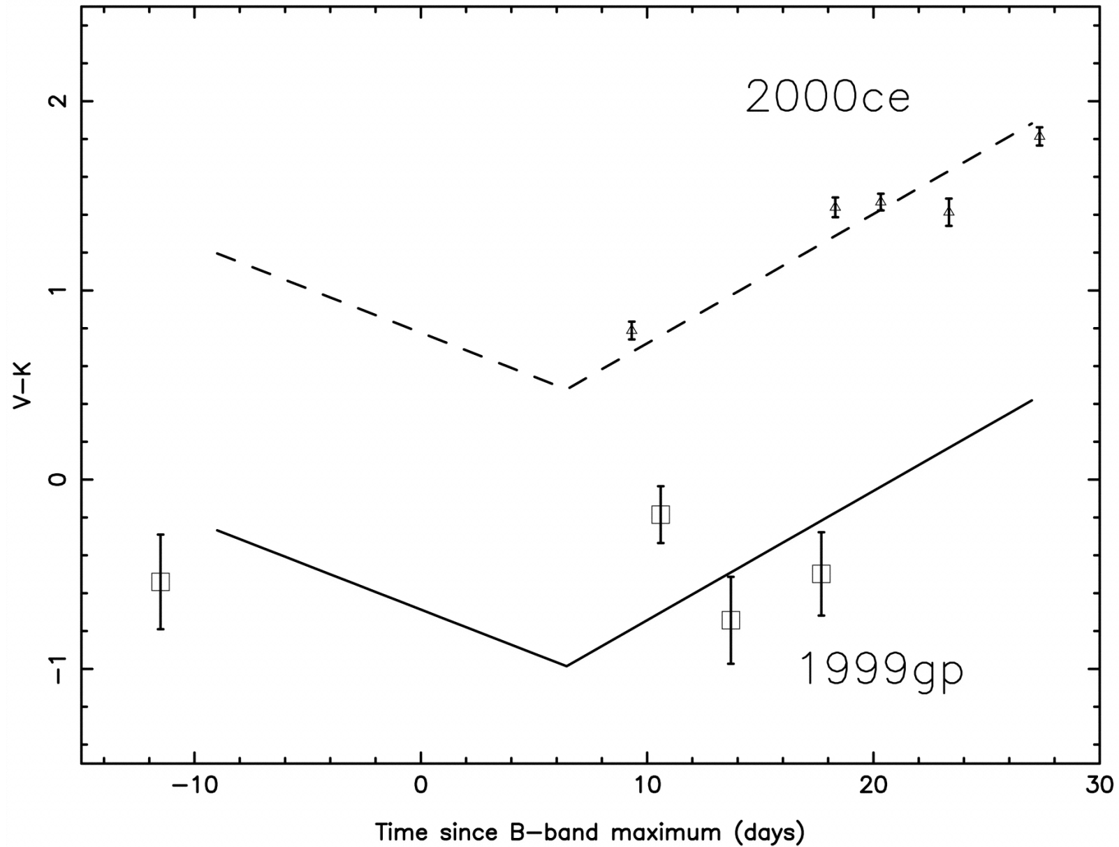
Fig. 14. from Optical and Infrared Photometry of the Type Ia Supernovae 1999da, 1999dk, 1999gp, 2000bk, and 2000ce Krisciunas et al. 2001 AJ 122 1616 doi:10.1086/322120 https://dx.doi.org/10.1086/322120 © 2001. The American Astronomical Society. All rights reserved. Printed in U.S.A.
