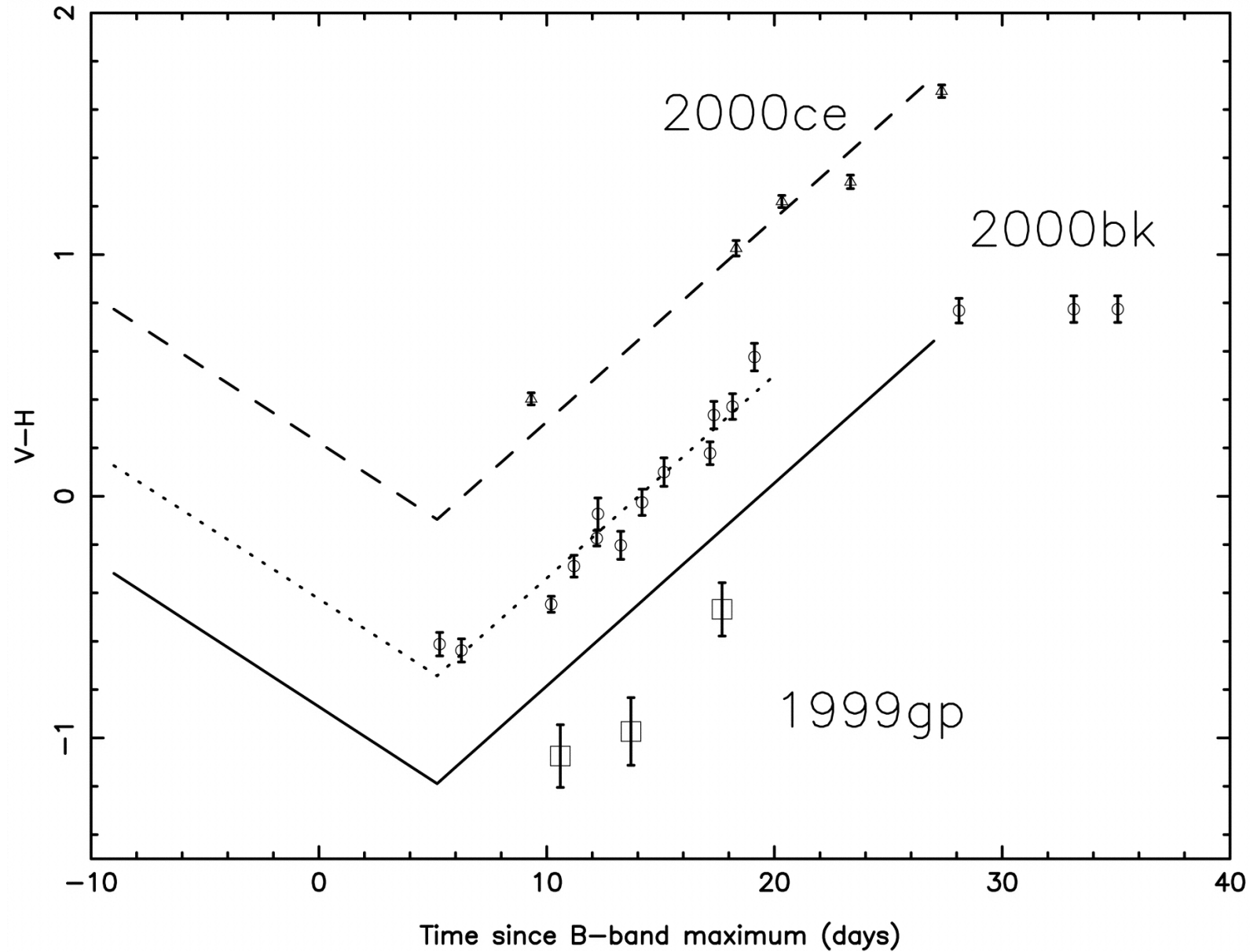
Fig. 13. from Optical and Infrared Photometry of the Type Ia Supernovae 1999da, 1999dk, 1999gp, 2000bk, and 2000ce Krisciunas et al. 2001 AJ 122 1616 doi:10.1086/322120 https://dx.doi.org/10.1086/322120 © 2001. The American Astronomical Society. All rights reserved. Printed in U.S.A.
