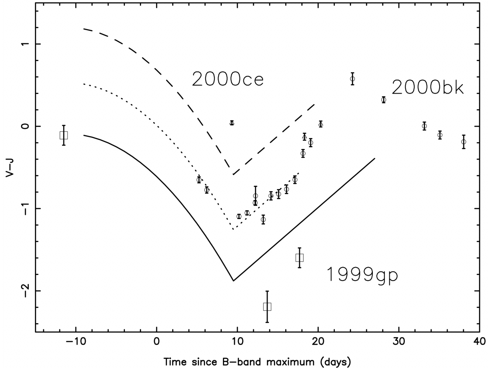
Fig. 12. from Optical and Infrared Photometry of the Type Ia Supernovae 1999da, 1999dk, 1999gp, 2000bk, and 2000ce Krisciunas et al. 2001 AJ 122 1616 doi:10.1086/322120 https://dx.doi.org/10.1086/322120 © 2001. The American Astronomical Society. All rights reserved. Printed in U.S.A.
