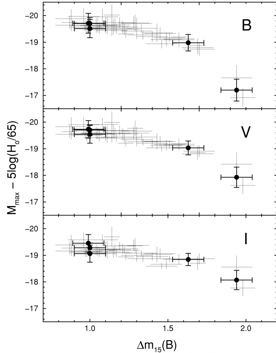
Fig. 11. from Optical and Infrared Photometry of the Type Ia Supernovae 1999da, 1999dk, 1999gp, 2000bk, and 2000ce Krisciunas et al. 2001 AJ 122 1616 doi:10.1086/322120 https://dx.doi.org/10.1086/322120
