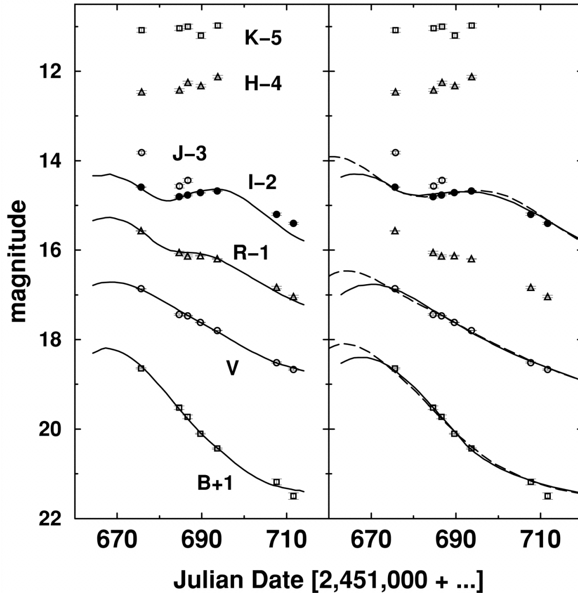
Fig. 10. from Optical and Infrared Photometry of the Type Ia Supernovae 1999da, 1999dk, 1999gp, 2000bk, and 2000ce Krisciunas et al. 2001 AJ 122 1616 doi:10.1086/322120 https://dx.doi.org/10.1086/322120
