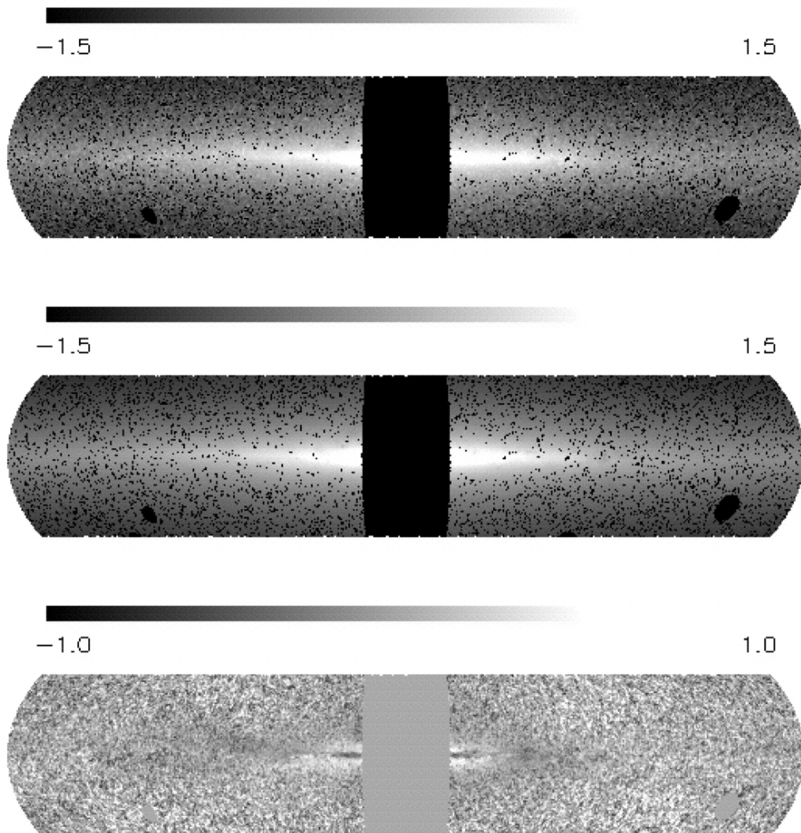
Fig. 9. from Threedimensional Structure of the Milky Way Disk: The Distribution of Stars and Dust beyond 0.35 R Drimmel & Spergel 2001 ApJ 556 181 doi:10.1086/321556 https://dx.doi.org/10.1086/321556 © 2001. The American Astronomical Society. All rights reserved. Printed in U.S.A.
