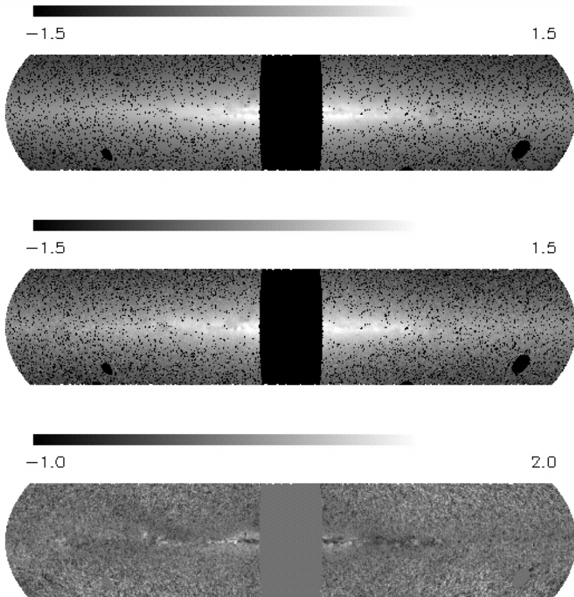
Fig. 8. from Threedimensional Structure of the Milky Way Disk: The Distribution of Stars and Dust beyond 0.35 R Drimmel & Spergel 2001 ApJ 556 181 doi:10.1086/321556 https://dx.doi.org/10.1086/321556 © 2001. The American Astronomical Society. All rights reserved. Printed in U.S.A.
