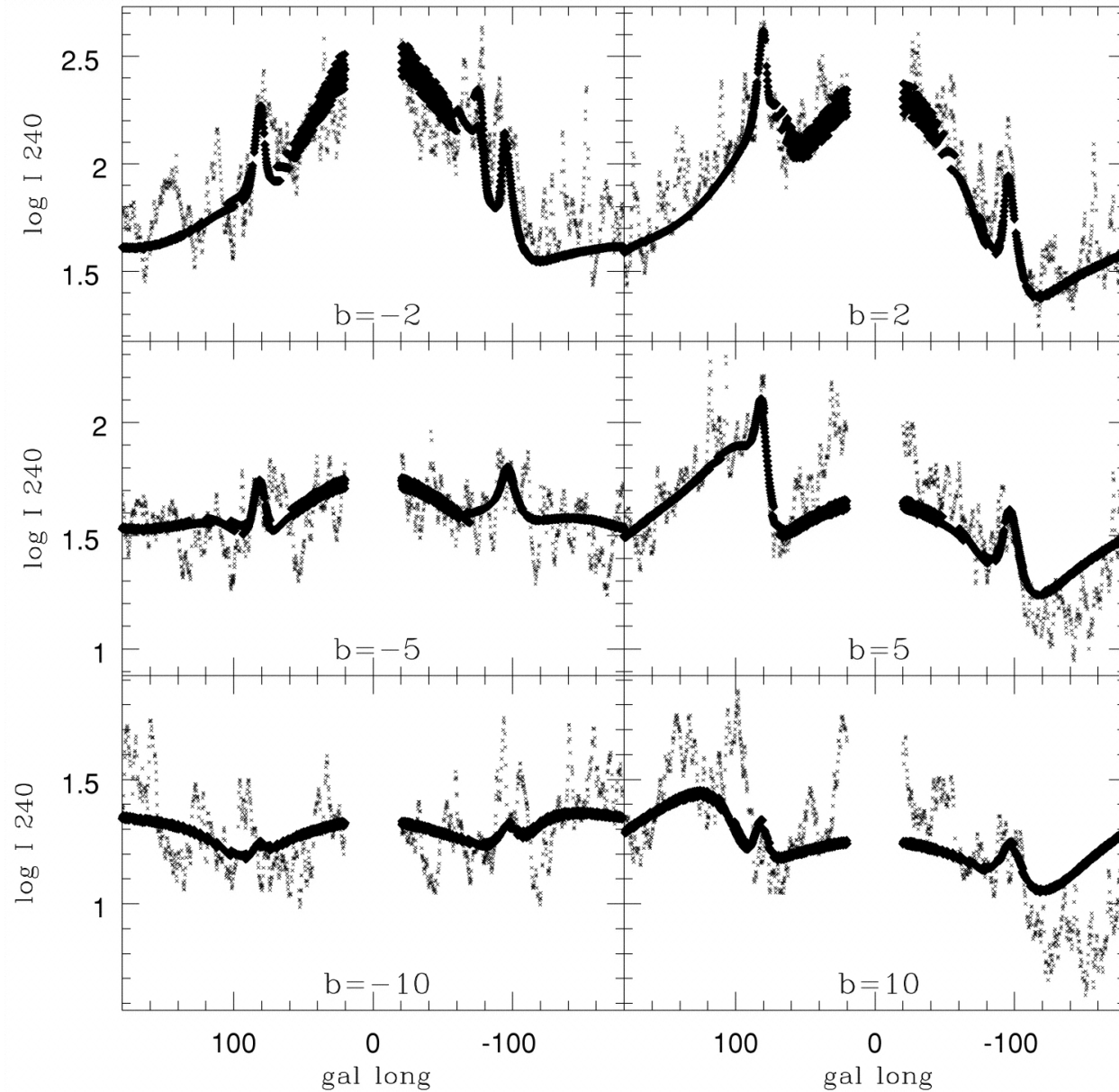
Fig. 6. from Threedimensional Structure of the Milky Way Disk: The Distribution of Stars and Dust beyond 0.35 R Drimmel & Spergel 2001 ApJ 556 181 doi:10.1086/321556 https://dx.doi.org/10.1086/321556 © 2001. The American Astronomical Society. All rights reserved. Printed in U.S.A.
