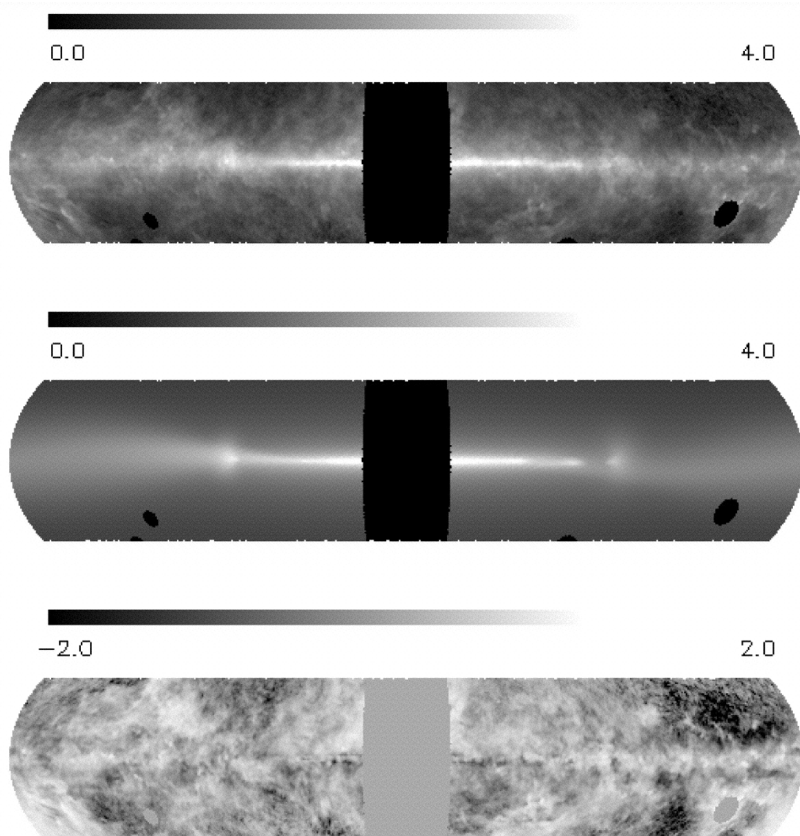
Fig. 4. from Threedimensional Structure of the Milky Way Disk: The Distribution of Stars and Dust beyond 0.35 R Drimmel & Spergel 2001 ApJ 556 181 doi:10.1086/321556 https://dx.doi.org/10.1086/321556
