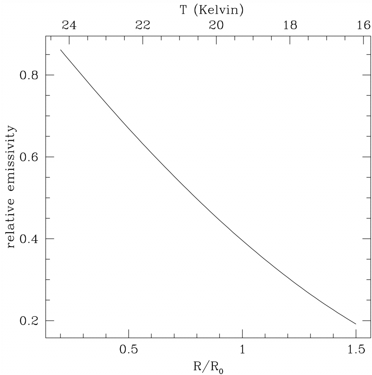
Fig. 3. from Threedimensional Structure of the Milky Way Disk: The Distribution of Stars and Dust beyond 0.35 R Drimmel & Spergel 2001 ApJ 556 181 doi:10.1086/321556 https://dx.doi.org/10.1086/321556
