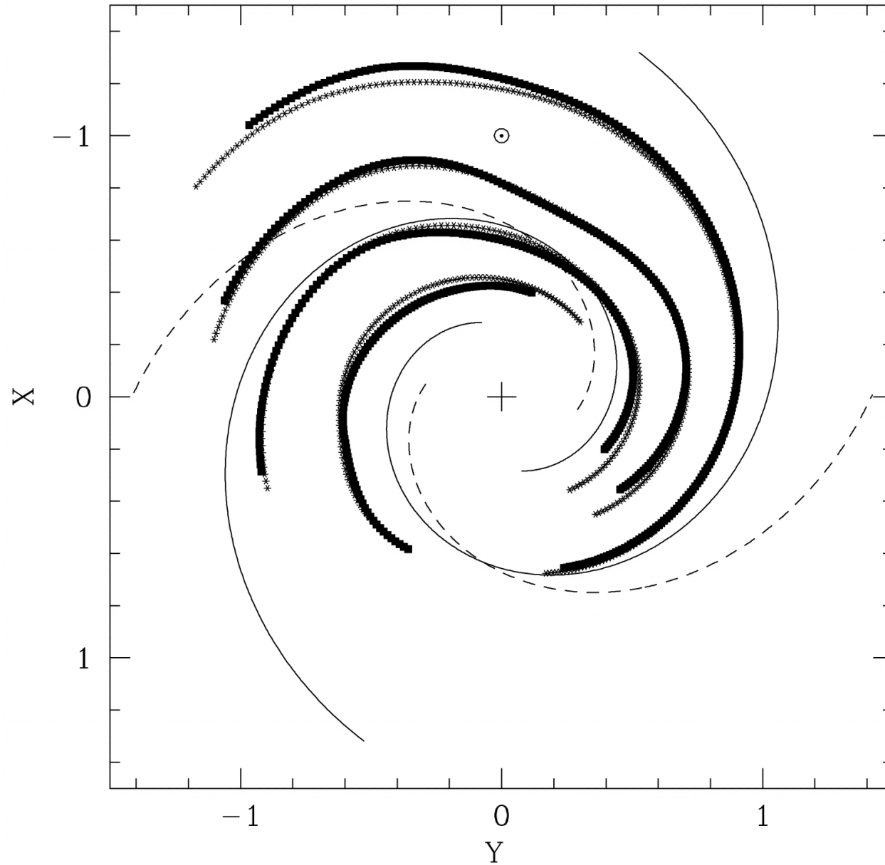
Fig. 19. from Threedimensional Structure of the Milky Way Disk: The Distribution of Stars and Dust beyond 0.35 R Drimmel & Spergel 2001 ApJ 556 181 doi:10.1086/321556 https://dx.doi.org/10.1086/321556 © 2001. The American Astronomical Society. All rights reserved. Printed in U.S.A.
