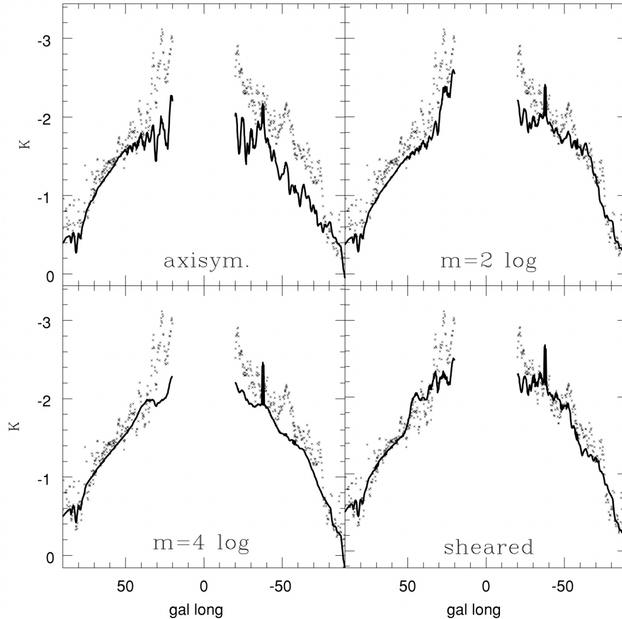
Fig. 18. from Threedimensional Structure of the Milky Way Disk: The Distribution of Stars and Dust beyond 0.35 R Drimmel & Spergel 2001 ApJ 556 181 doi:10.1086/321556 https://dx.doi.org/10.1086/321556 © 2001. The American Astronomical Society. All rights reserved. Printed in U.S.A.
