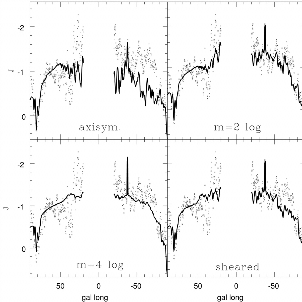
Fig. 17. from Threedimensional Structure of the Milky Way Disk: The Distribution of Stars and Dust beyond 0.35 R Drimmel & Spergel 2001 ApJ 556 181 doi:10.1086/321556 https://dx.doi.org/10.1086/321556 © 2001. The American Astronomical Society. All rights reserved. Printed in U.S.A.
