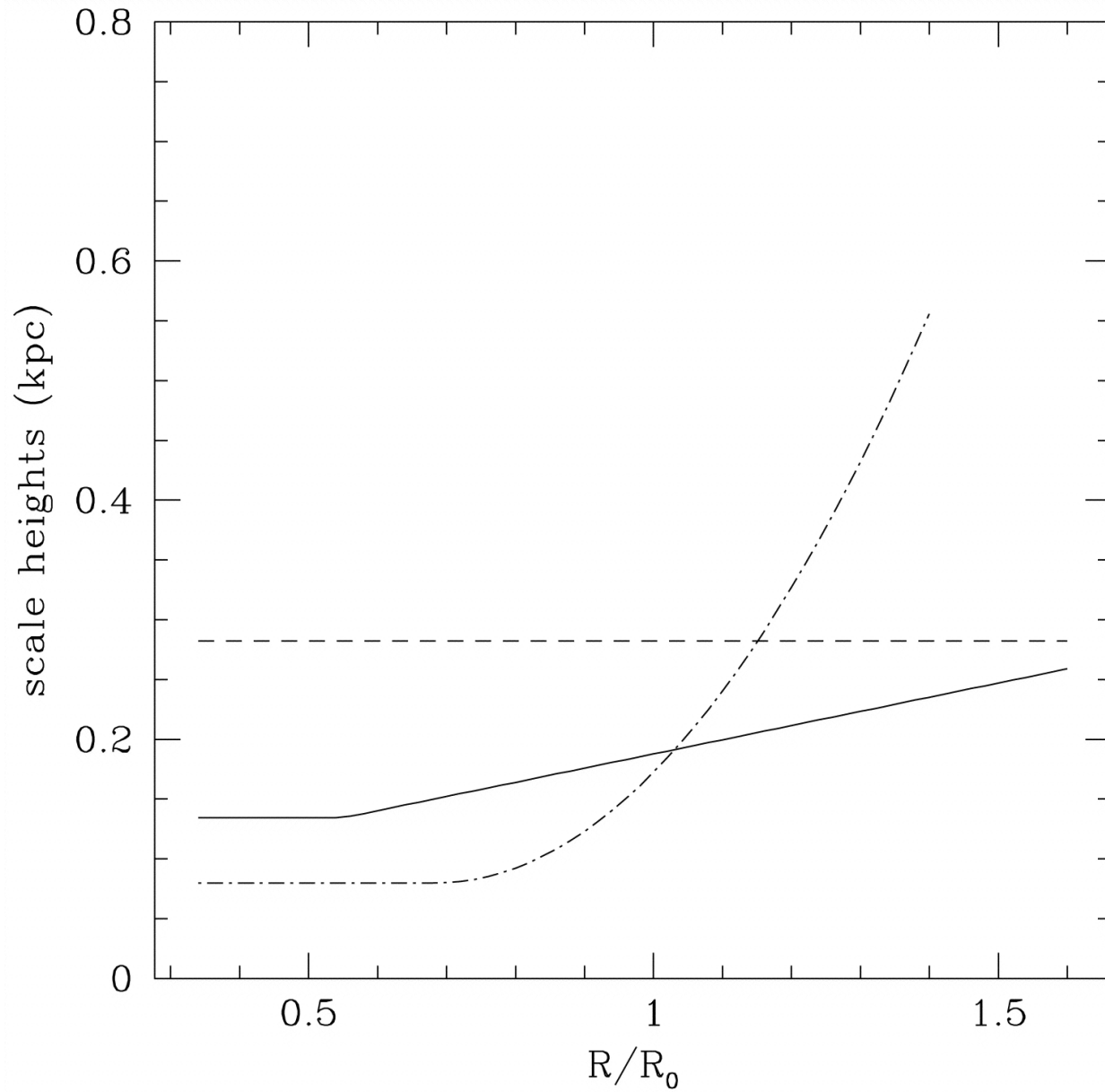
Fig. 16. from Threedimensional Structure of the Milky Way Disk: The Distribution of Stars and Dust beyond 0.35 R Drimmel & Spergel 2001 ApJ 556 181 doi:10.1086/321556 https://dx.doi.org/10.1086/321556 © 2001. The American Astronomical Society. All rights reserved. Printed in U.S.A.
