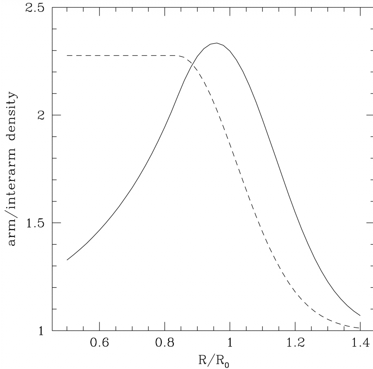
Fig. 15. from Threedimensional Structure of the Milky Way Disk: The Distribution of Stars and Dust beyond 0.35 R Drimmel & Spergel 2001 ApJ 556 181 doi:10.1086/321556 https://dx.doi.org/10.1086/321556 © 2001. The American Astronomical Society. All rights reserved. Printed in U.S.A.
