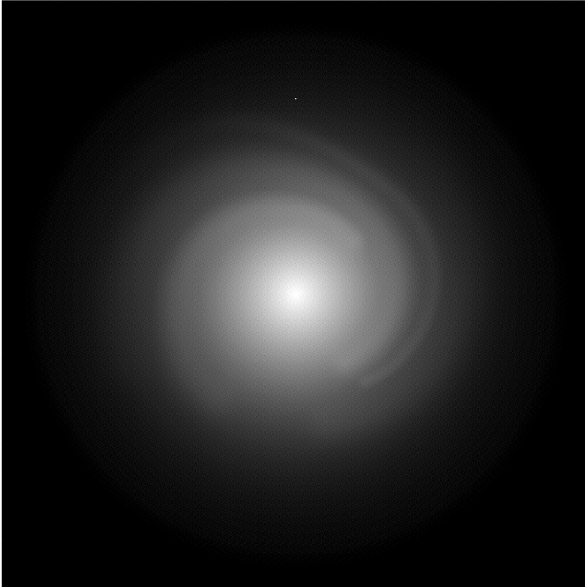
Fig. 14. from Threedimensional Structure of the Milky Way Disk: The Distribution of Stars and Dust beyond 0.35 R Drimmel & Spergel 2001 ApJ 556 181 doi:10.1086/321556 https://dx.doi.org/10.1086/321556 © 2001. The American Astronomical Society. All rights reserved. Printed in U.S.A.
