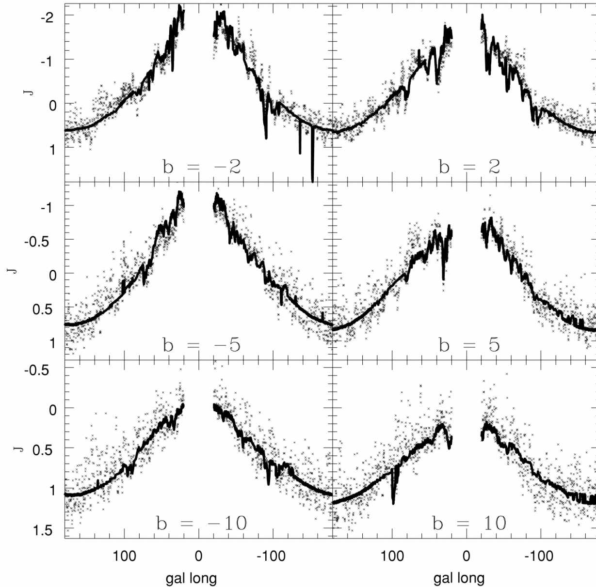
Fig. 11. from Threedimensional Structure of the Milky Way Disk: The Distribution of Stars and Dust beyond 0.35 R Drimmel & Spergel 2001 ApJ 556 181 doi:10.1086/321556 https://dx.doi.org/10.1086/321556 © 2001. The American Astronomical Society. All rights reserved. Printed in U.S.A.
