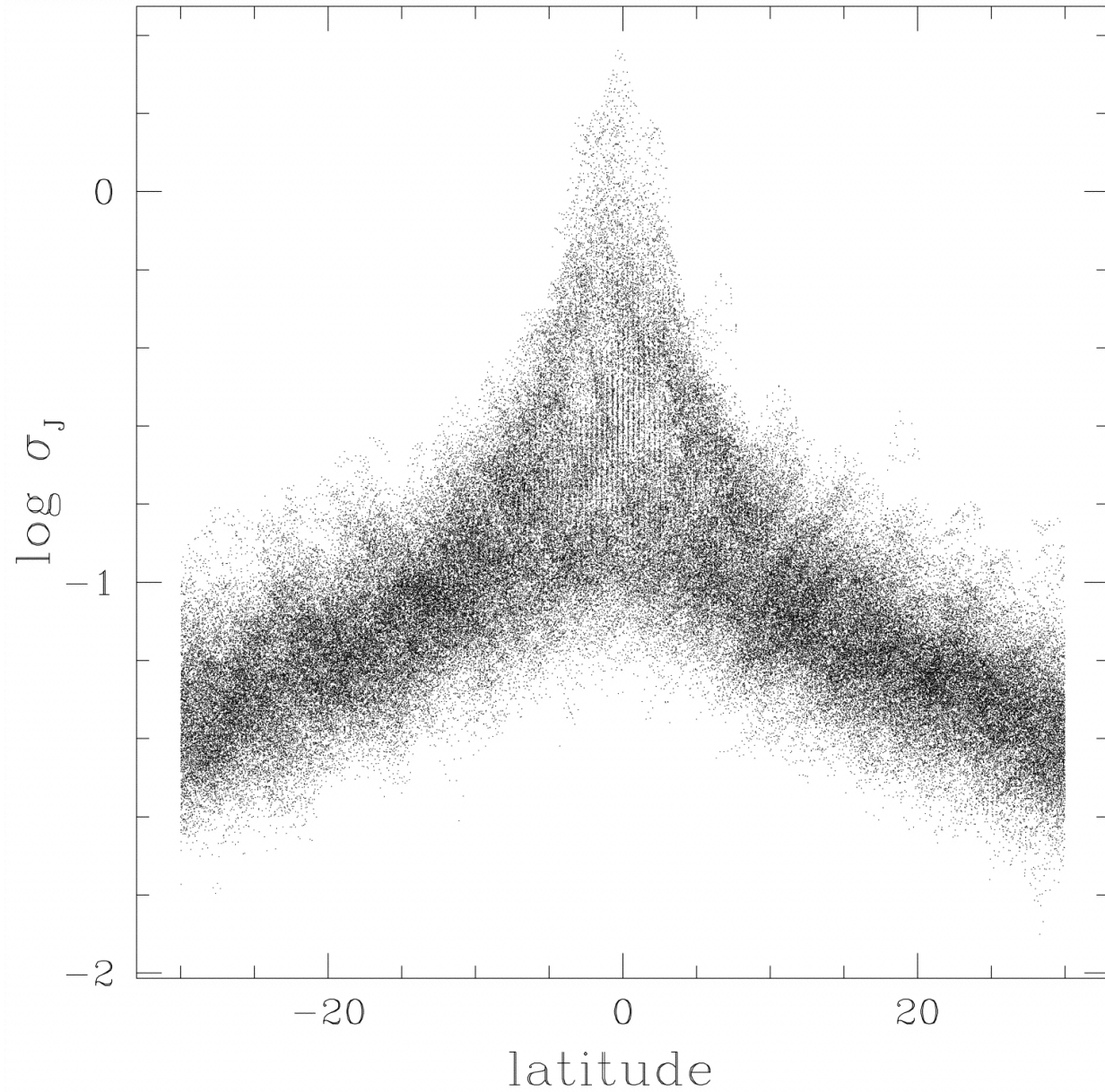
Fig. 1. from Threedimensional Structure of the Milky Way Disk: The Distribution of Stars and Dust beyond 0.35 R Drimmel & Spergel 2001 ApJ 556 181 doi:10.1086/321556 https://dx.doi.org/10.1086/321556 © 2001. The American Astronomical Society. All rights reserved. Printed in U.S.A.
