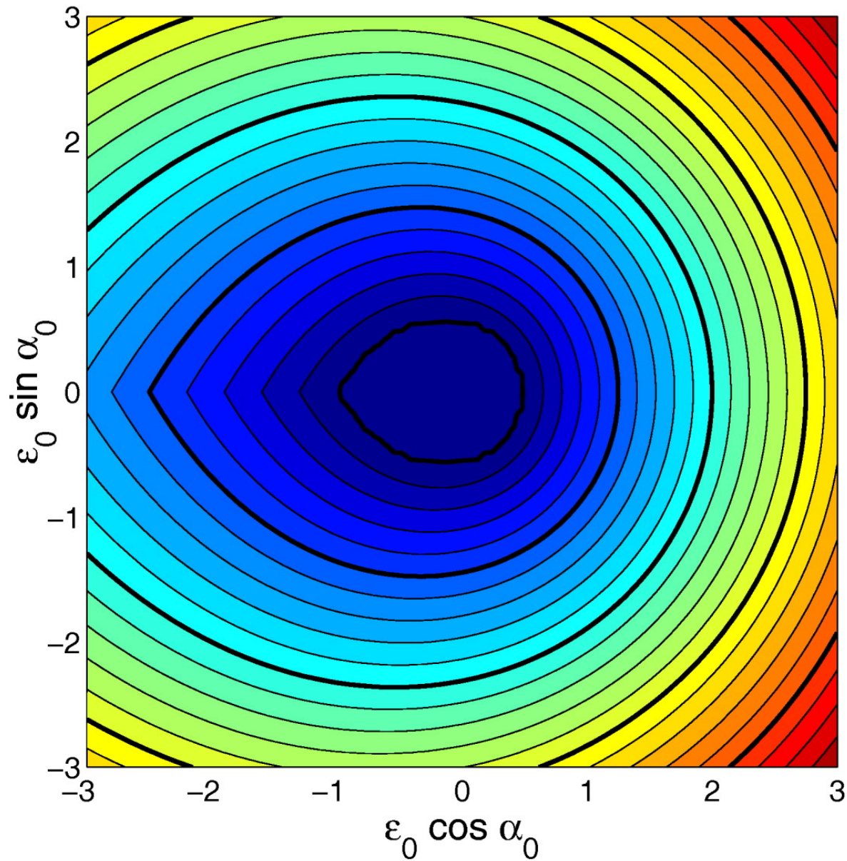
Fig. 3. from On Local Approximations to the Nonlinear Evolution of LargeScale Structure Makler, Kodama, & Calvão 2001 ApJ 557 88 doi:10.1086/321551 https://dx.doi.org/10.1086/321551 © 2001. The American Astronomical Society. All rights reserved. Printed in U.S.A.
