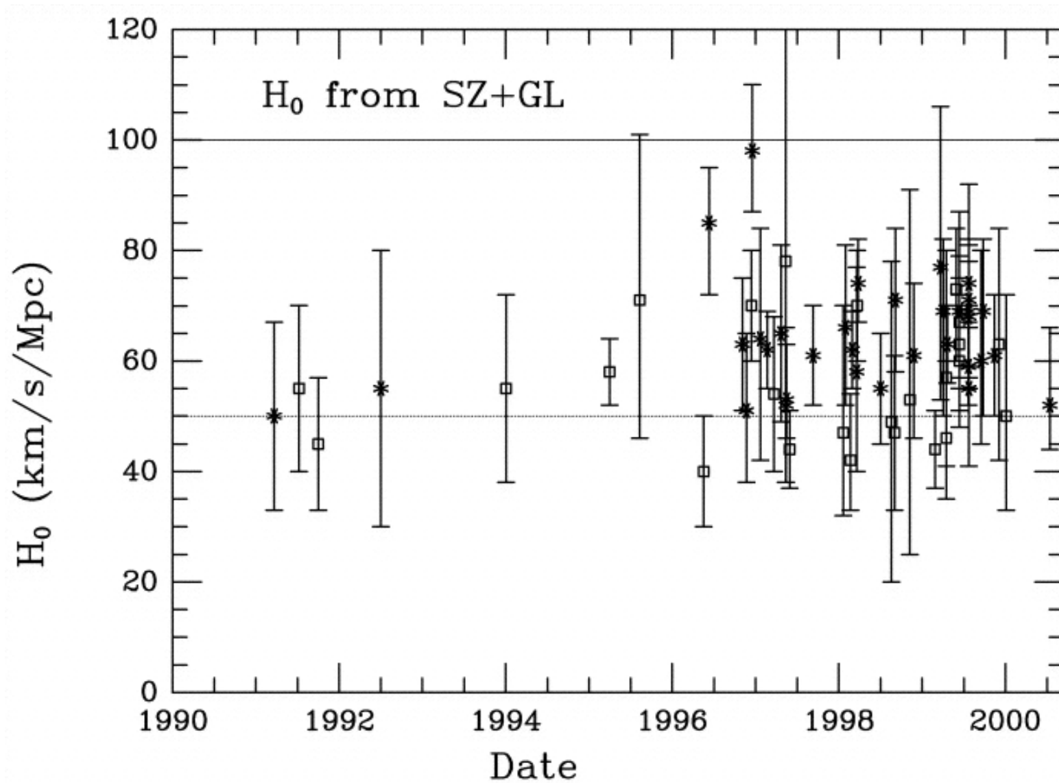
Fig. 7. from Final Results from the Hubble Space Telescope Key Project to Measure the Hubble Constant Freedman et al. 2001 ApJ 553 47 doi:10.1086/320638 https://dx.doi.org/10.1086/320638 © 2001. The American Astronomical Society. All rights reserved. Printed in U.S.A.
